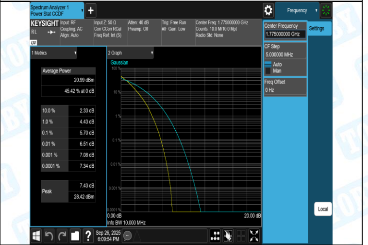
Band66-10MHz-16QAM-132322-1RB#0-PASS
