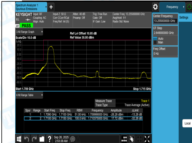
Band66-5MHz-16QAM-131997-25RB#0-PASS
