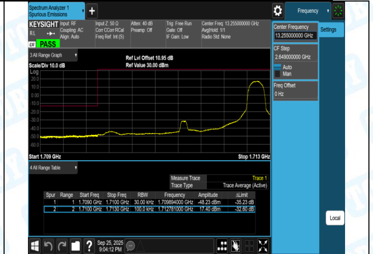
Band66-3MHz-16QAM-132657-1RB#0-PASS
