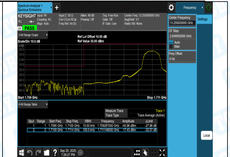
Band66-1.4MHz-16QAM-132665-1RB#0-PASS
