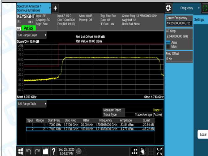
Band66-3MHz-QPSK-132657-1RB#14-PASS
