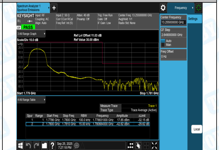
Band66-1.4MHz-16QAM-132665-6RB#0-PASS
