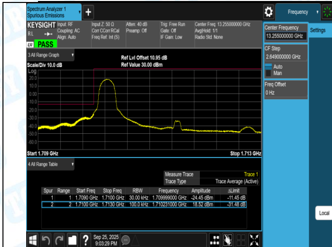
Band66-3MHz-QPSK-131987-15RB#0-PASS
