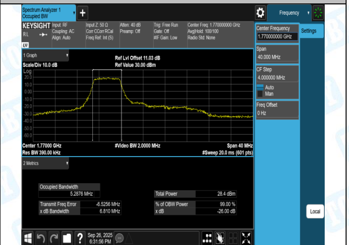
Band66-20MHz-16QAM-132572-27RB#0-PASS
