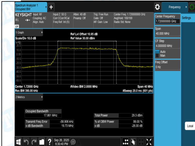
Band66-20MHz-QPSK-132572-100RB#0-PASS
