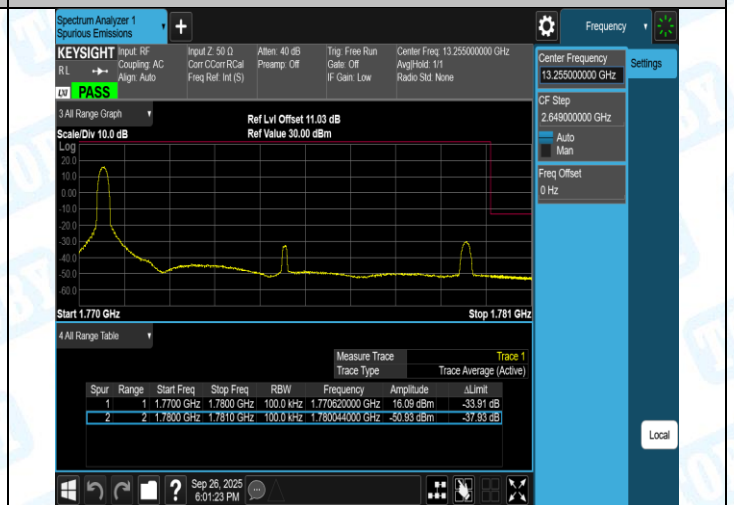
Band66-10MHz-QPSK-132622-50RB#0-PASS
