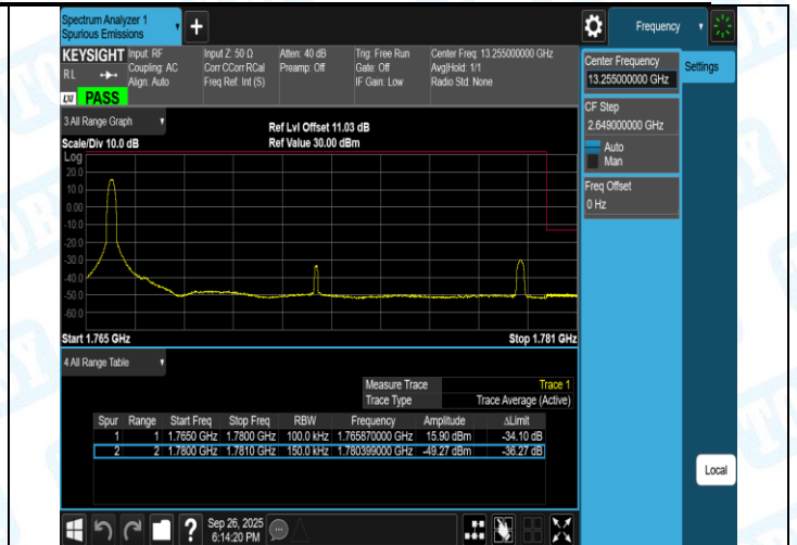
Band66-15MHz-QPSK-132597-75RB#0-PASS
