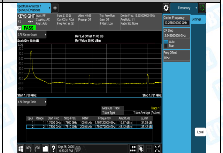
Band66-20MHz-QPSK-132572-100RB#0-PASS
