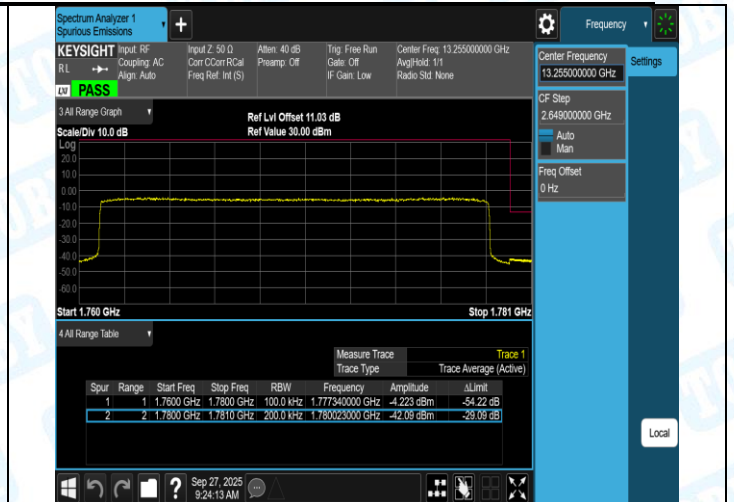
Band66-20MHz-16QAM-132072-1RB#99-PASS
