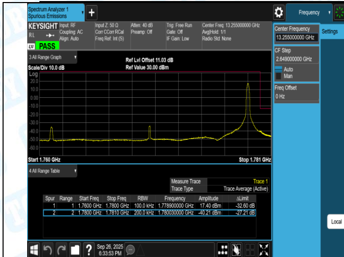
Band66-20MHz-16QAM-132072-1RB#0-PASS
