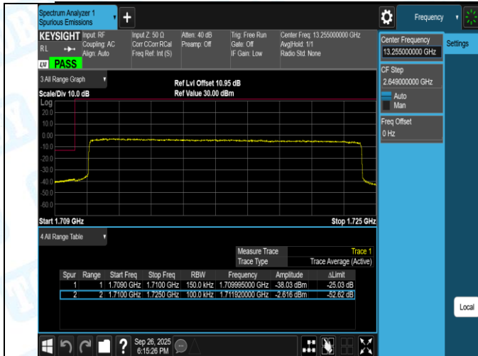
Band66-15MHz-QPSK-132597-1RB#74-PASS
