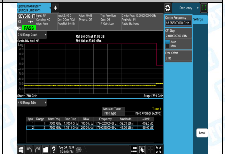
Band66-20MHz-16QAM-132572-1RB#99-PASS
