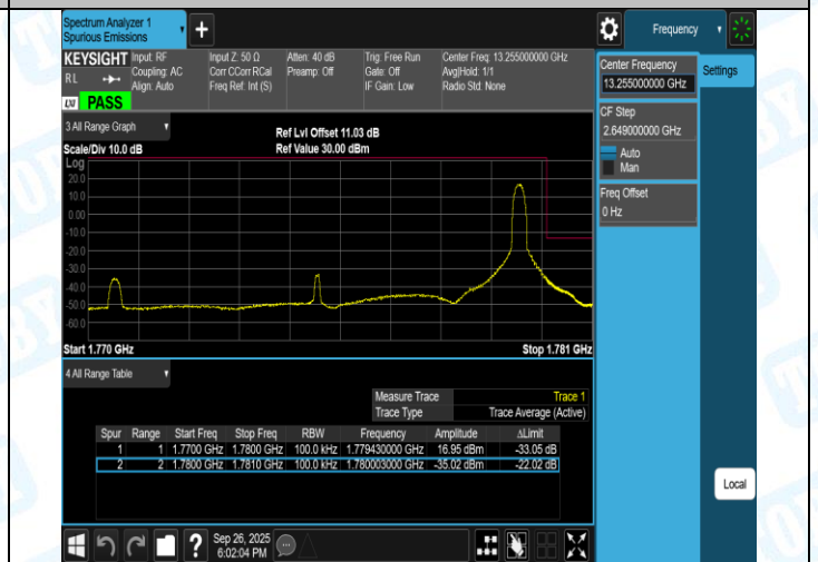
Band66-15MHz-QPSK-132047-1RB#74-PASS
