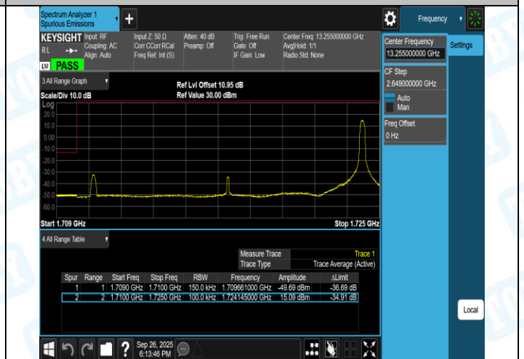
Band66-15MHz-QPSK-132597-1RB#0-PASS
