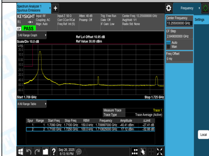
Band66-15MHz-QPSK-132047-75RB#0-PASS
