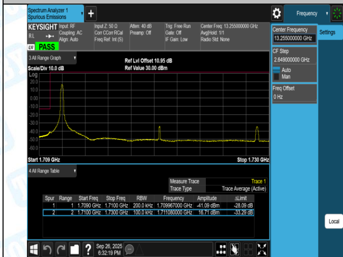
Band66-20MHz-QPSK-132072-100RB#0-PASS
