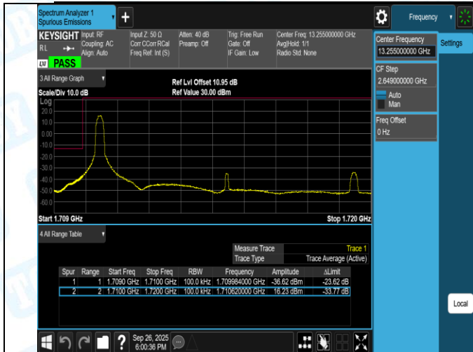
Band66-10MHz-16QAM-132622-1RB#0-PASS
