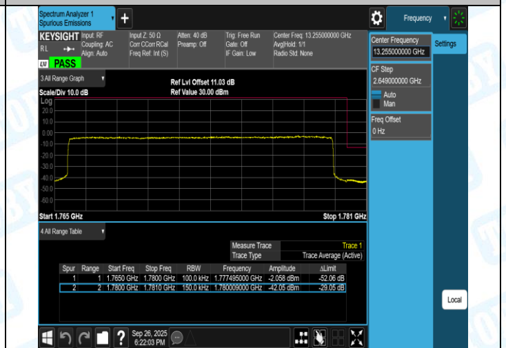
Band66-15MHz-16QAM-132047-1RB#74-PASS
