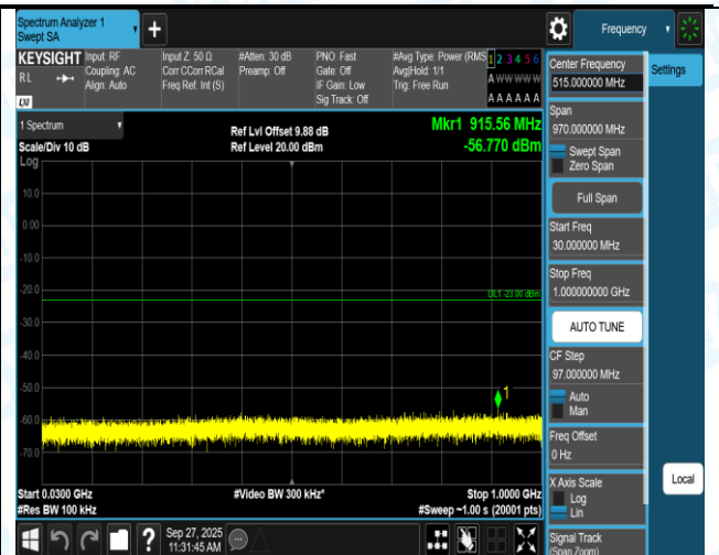
Band66-1.4MHz-QPSK-131979-1RB#5-3000~20000-PASS
