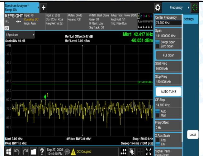
Band66-3MHz-QPSK-132322-15RB#0-30-1000-PASS
