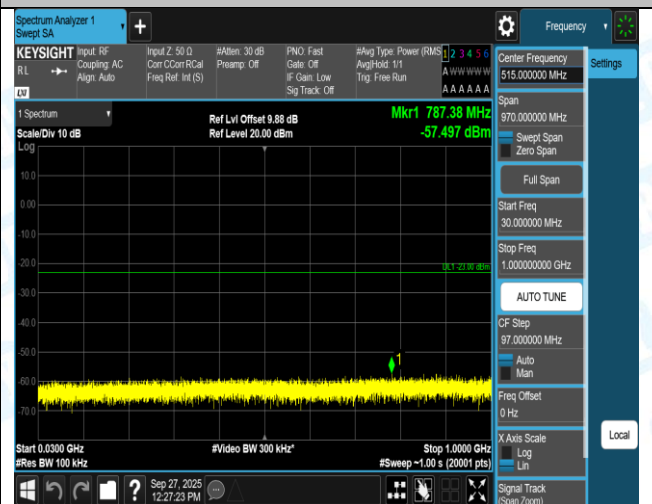
Band66-3MHz-16QAM-131987-1RB#0-3000~20000-PASS
