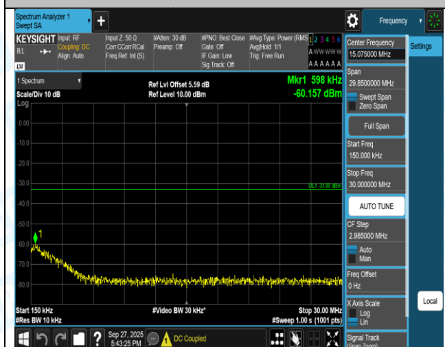
Band66-5MHz-QPSK-132322-1RB#0-1000~3000-PASS
