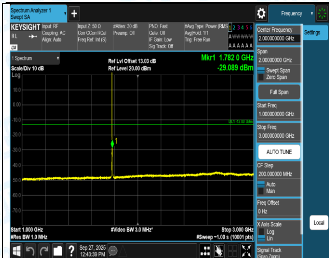
Band66-3MHz-16QAM-132657-1RB#14-0.009-0.15-PASS
