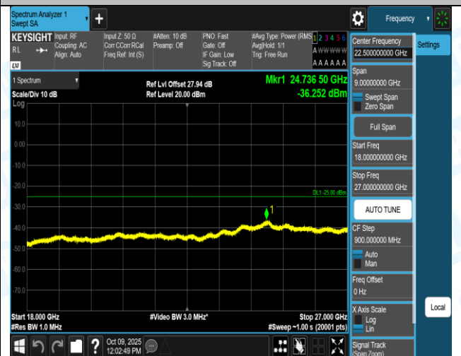
Band7-20MHz-16QAM-20850-1RB#99-0.15~30-PASS
