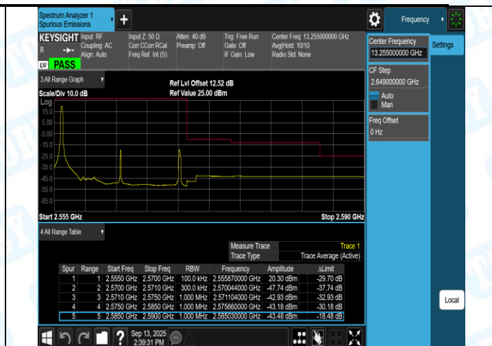
Band7-15MHz-QPSK-21375-75RB#0-PASS
