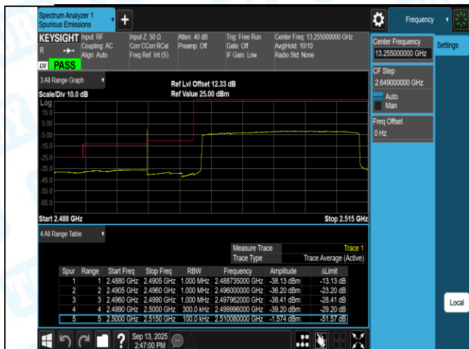
Band7-15MHz-QPSK-21375-1RB#74-PASS
