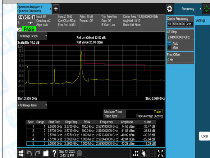
Band7-15MHz-16QAM-20825-1RB#0-PASS
