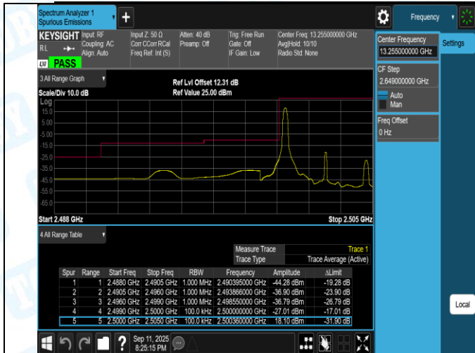
Band7-5MHz-16QAM-20775-25RB#0-PASS
