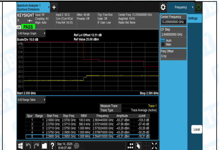
Band7-20MHz-16QAM-20850-1RB#99-PASS
