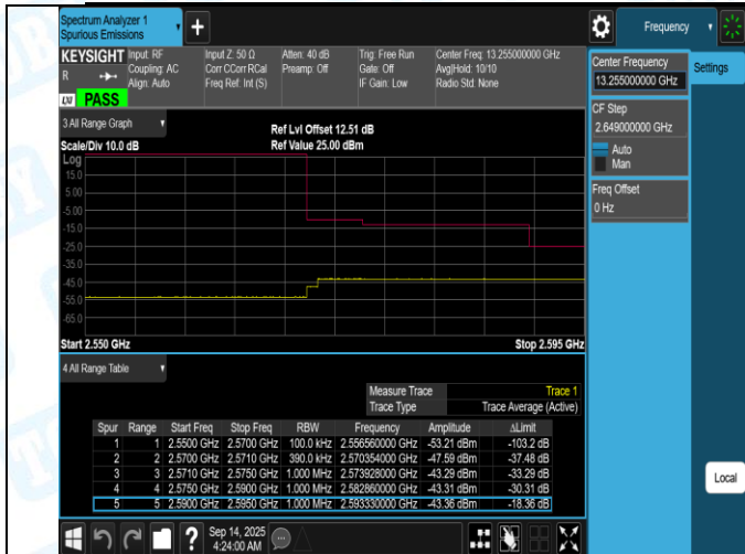
Band7-20MHz-16QAM-20850-1RB#0-PASS
