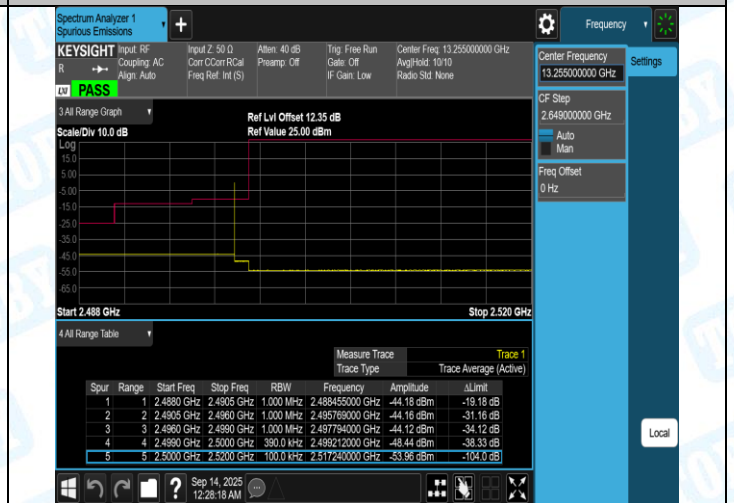
Band7-20MHz-QPSK-20850-100RB#99-PASS
