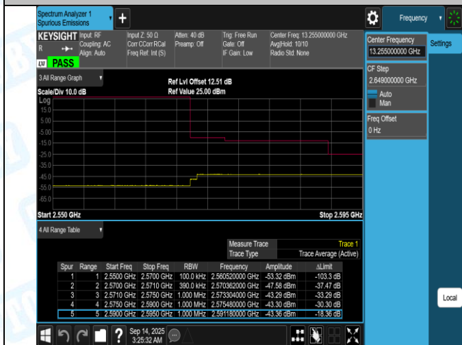
Band7-20MHz-16QAM-21350-1RB#0-PASS
