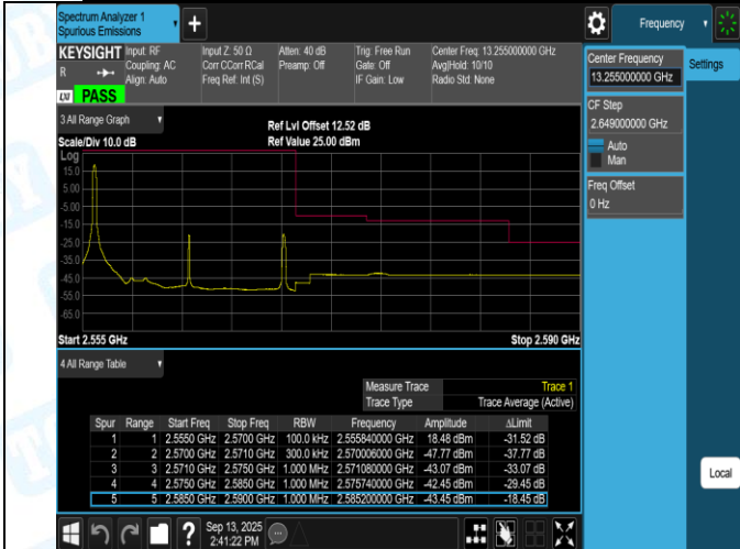
Band7-20MHz-QPSK-20850-1RB#0-PASS
