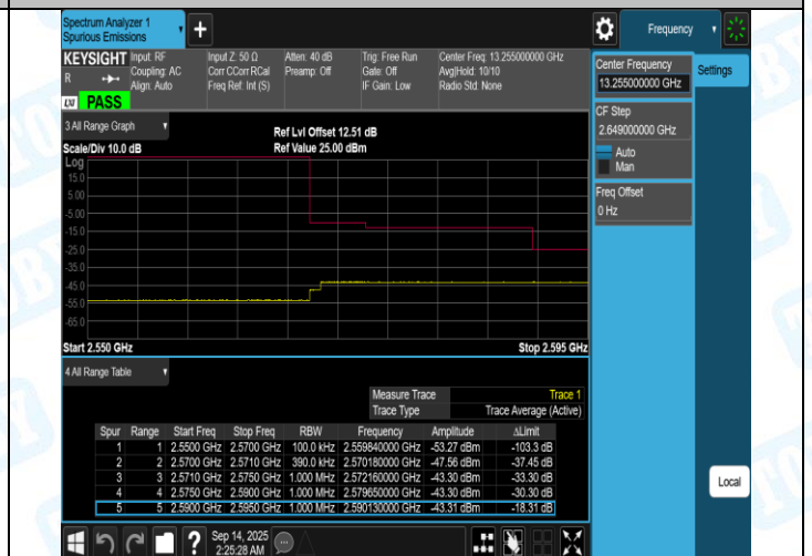
Band7-20MHz-QPSK-21350-100RB#0-PASS
