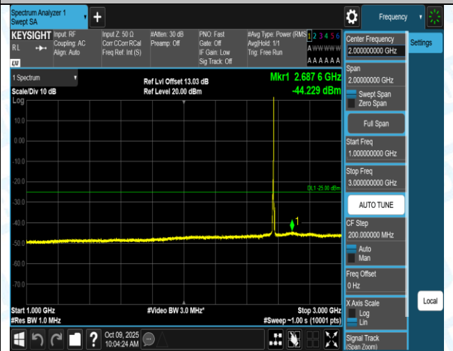
Band7-5MHz-QPSK-21425-1RB#24-18000~27000-PASS
