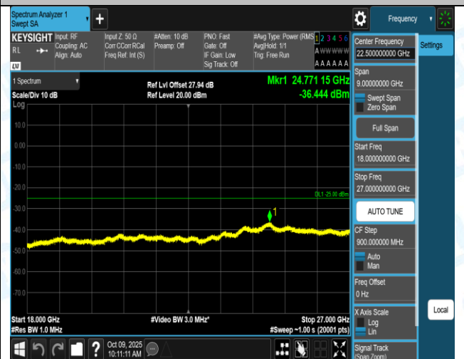
Band7-5MHz-16QAM-21425-25RB#0-0.15~30-PASS
