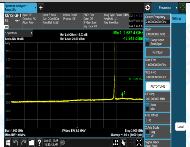
Band7-10MHz-QPSK-21400-1RB#0-18000~27000-PASS
