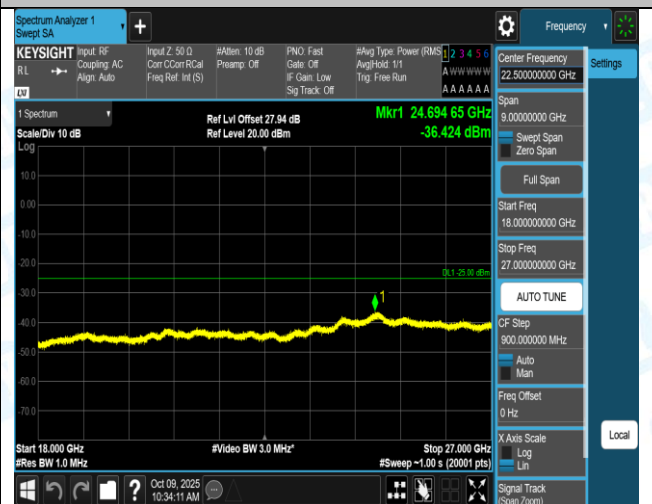
Band7-10MHz-QPSK-21400-1RB#49-0.15~30-PASS
