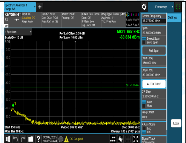
Band7-10MHz-16QAM-21400-1RB#49-1000~3000-PASS
