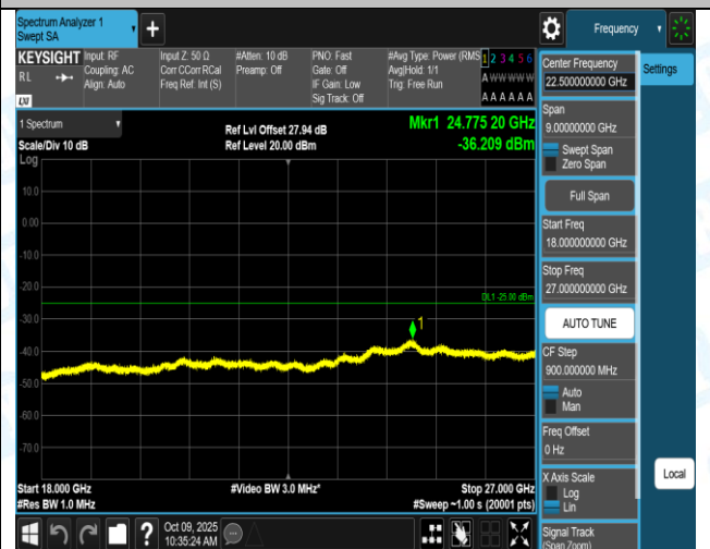
Band7-10MHz-16QAM-21400-1RB#49-0.15~30-PASS
