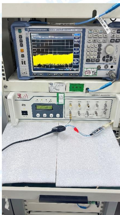
Photo of Setup for Conducted Measurement
