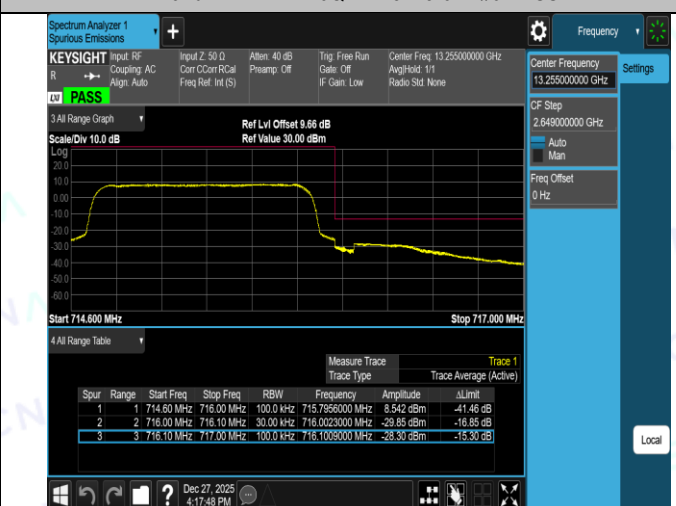
Band12-3MHz-QPSK-23025-1RB#14-PASS
