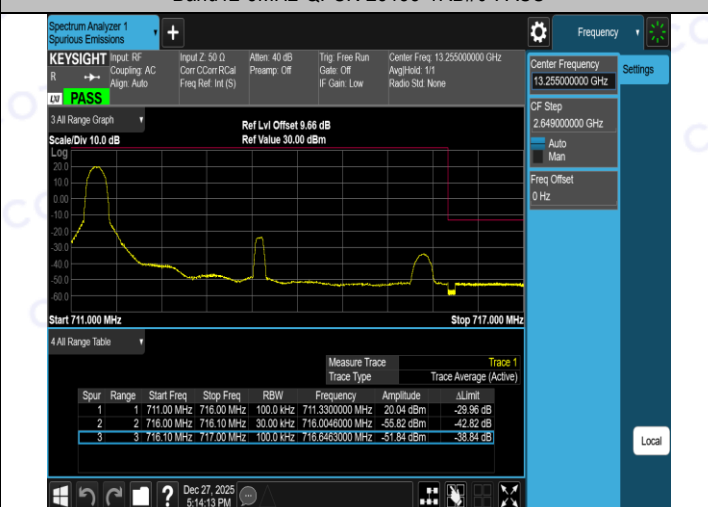
Band12-5MHz-QPSK-23155-25RB#0-PASS
