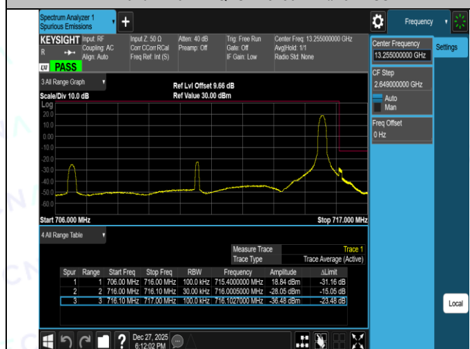
Band12-10MHz-16QAM-23060-1RB#0-PASS
