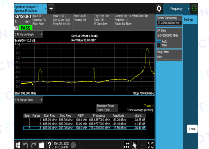
Band12-10MHz-QPSK-23130-1RB#0-PASS
