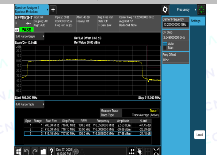
Band12-10MHz-16QAM-23060-1RB#49-PASS
