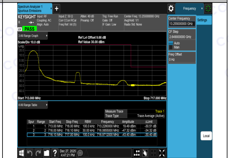
Band12-3MHz-QPSK-23165-15RB#0-PASS
