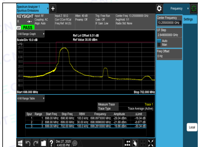
Band12-3MHz-16QAM-23025-15RB#0-PASS
