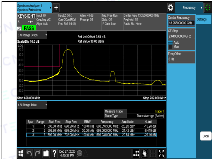
Band12-3MHz-QPSK-23025-15RB#0-PASS
