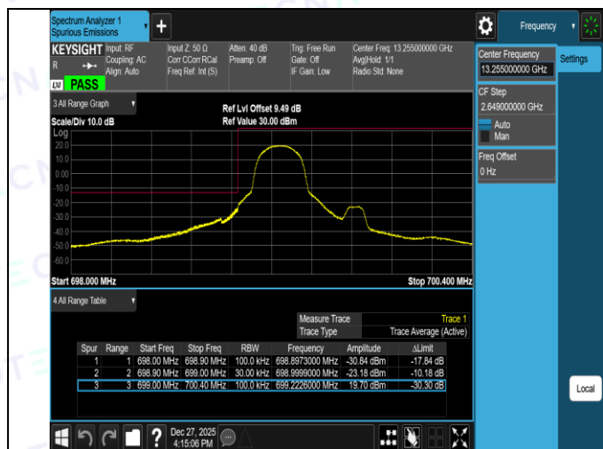
Band12-1.4MHz-16QAM-23017-6RB#0-PASS
