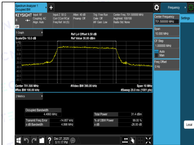
Band12-5MHz-QPSK-23155-25RB#0-PASS
