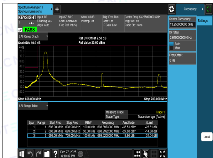
Band12-10MHz-16QAM-23130-1RB#0-PASS
