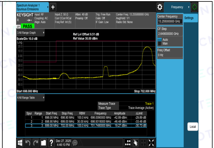
Band12-3MHz-QPSK-23165-1RB#0-PASS
