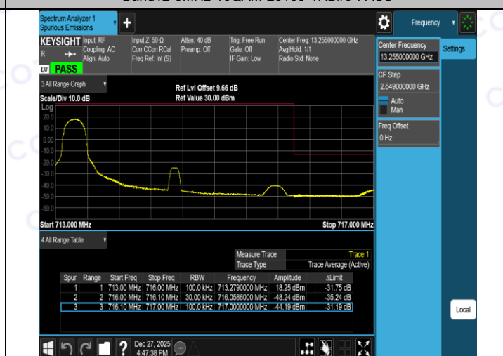
Band12-3MHz-16QAM-23165-15RB#0-PASS
