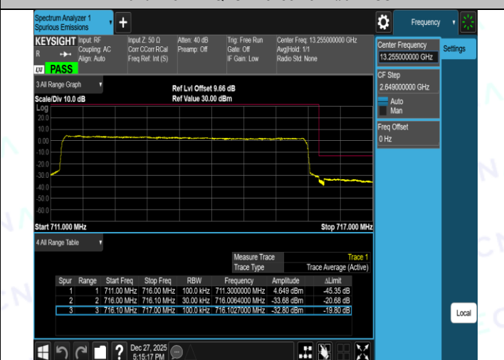
Band12-5MHz-16QAM-23035-1RB#24-PASS
