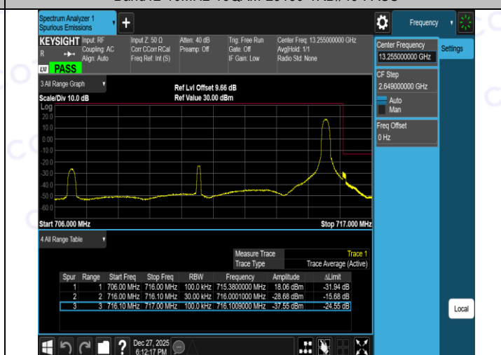
Band12-10MHz-16QAM-23130-1RB#49-PASS
