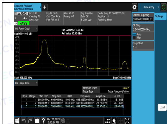
Band12-5MHz-QPSK-23035-25RB#0-PASS
