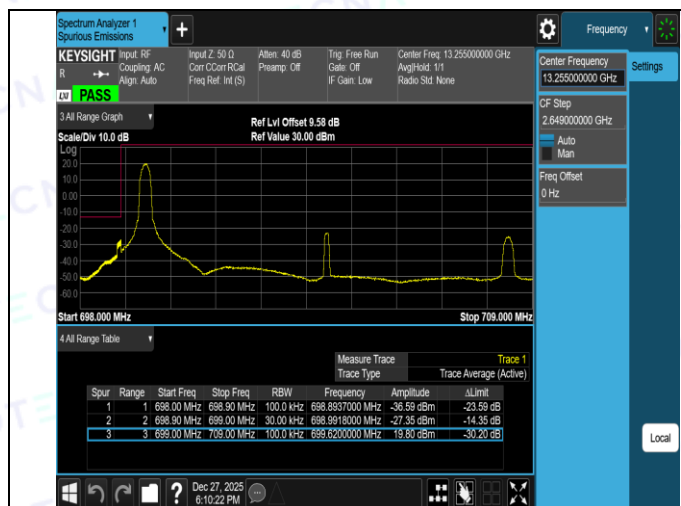
Band12-10MHz-QPSK-23060-50RB#0-PASS
