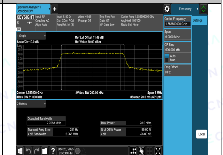
Band4-5MHz-QPSK-20175-25RB#0-PASS
