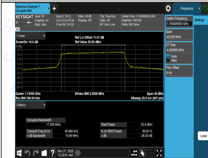
Band4-20MHz-16QAM-20175-27RB#0-PASS
