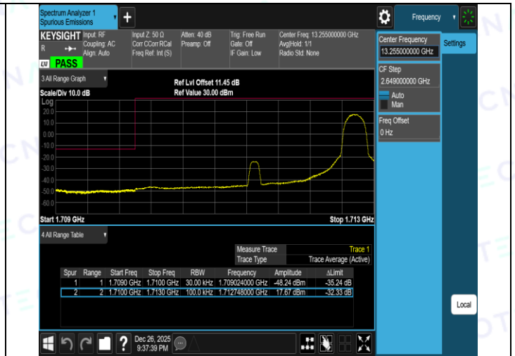
Band4-3MHz-QPSK-20385-1RB#0-PASS
