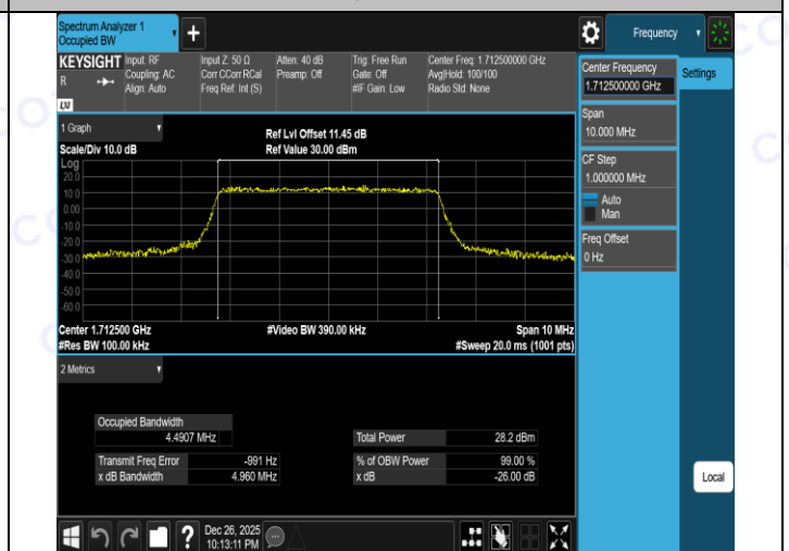
Band4-5MHz-16QAM-20375-25RB#0-PASS
