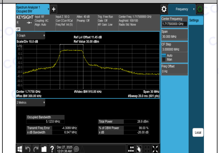
Band4-15MHz-16QAM-20325-27RB#0-PASS
