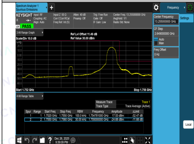
Band4-3MHz-16QAM-19965-1RB#0-PASS
