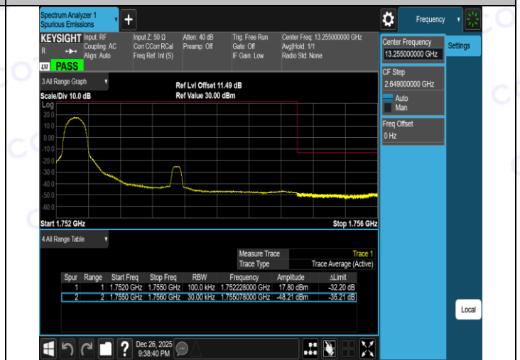
Band4-3MHz-QPSK-20385-15RB#0-PASS
