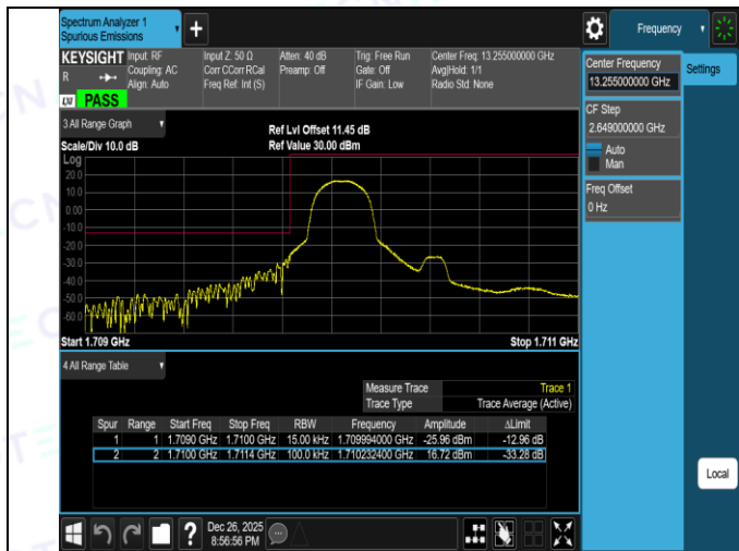
Band4-1.4MHz-16QAM-19957-6RB#0-PASS
