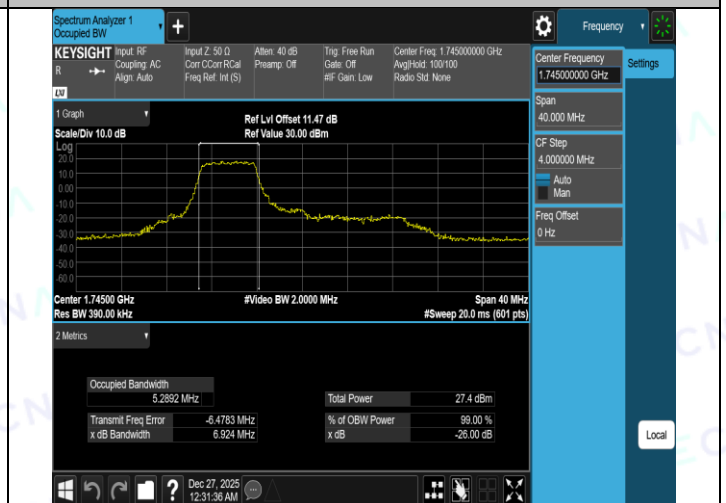
Band4-20MHz-16QAM-20300-27RB#0-PASS
