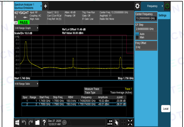
Band4-15MHz-QPSK-20325-75RB#0-PASS
