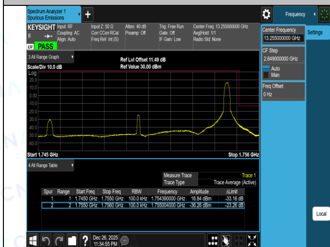
Band4-10MHz-16QAM-20000-1RB#0-PASS
