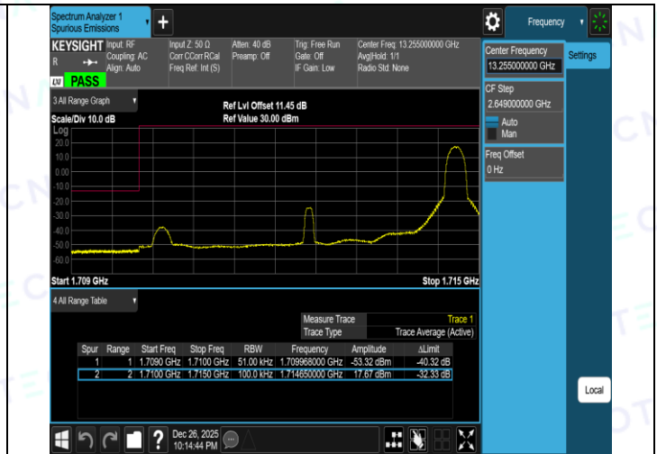
Band4-5MHz-QPSK-20375-1RB#0-PASS
