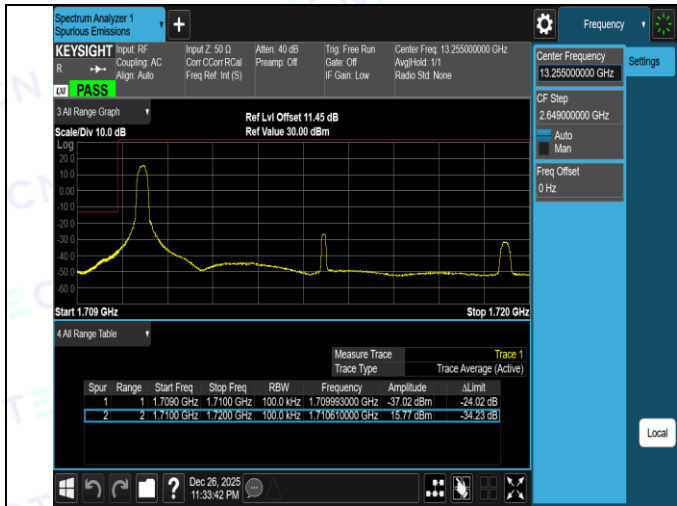
Band4-10MHz-16QAM-20350-1RB#0-PASS
