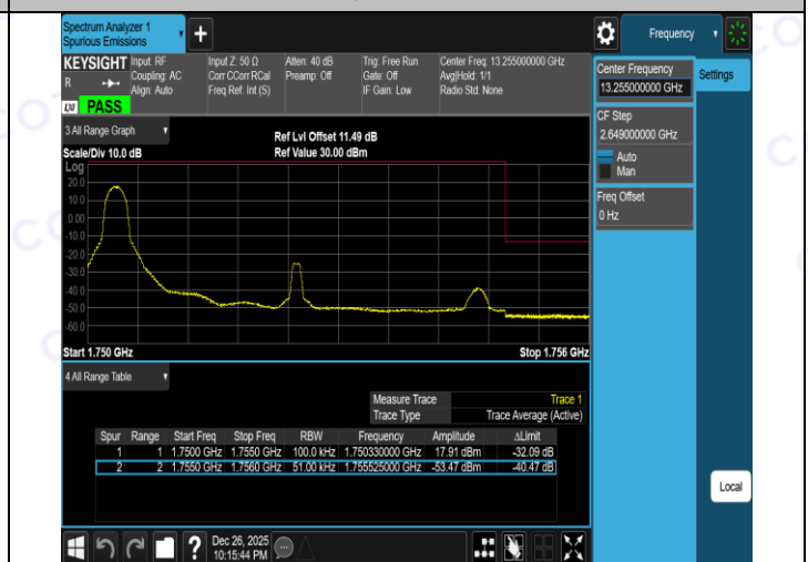
Band4-5MHz-QPSK-20375-25RB#0-PASS
