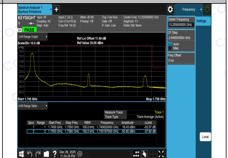
Band4-10MHz-QPSK-20350-50RB#0-PASS
