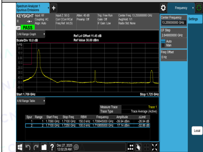
Band4-15MHz-QPSK-20025-75RB#0-PASS
