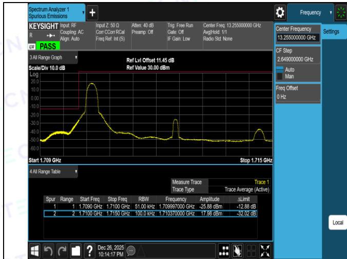
Band4-5MHz-QPSK-19975-25RB#0-PASS
