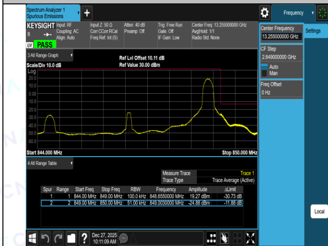
Band5-5MHz-16QAM-20425-1RB#0-PASS
