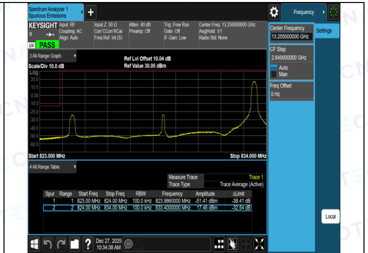
Band5-10MHz-QPSK-20600-1RB#0-PASS
