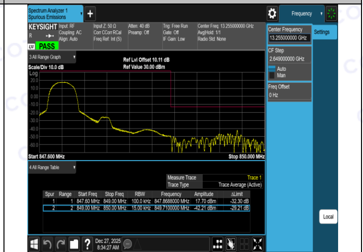
Band5-1.4MHz-16QAM-20643-6RB#0-PASS
