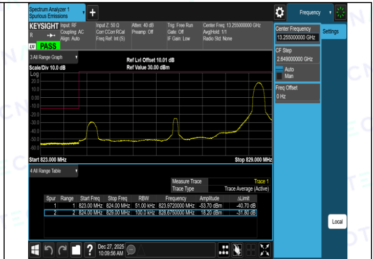
Band5-5MHz-16QAM-20625-1RB#0-PASS
