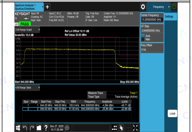
Band5-5MHz-16QAM-20425-1RB#24-PASS
