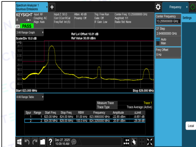
Band5-5MHz-QPSK-20425-25RB#0-PASS
