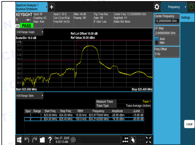
Band5-1.4MHz-16QAM-20407-6RB#0-PASS
