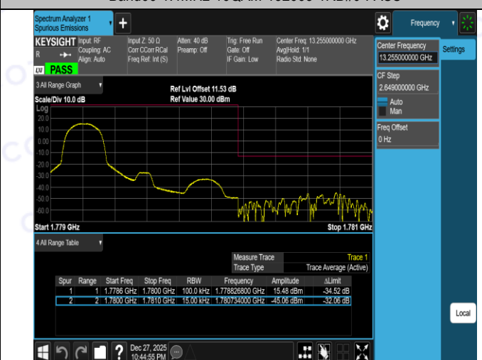
Band66-1.4MHz-16QAM-132665-6RB#0-PASS
