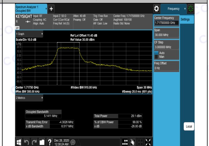
Band66-15MHz-16QAM-132597-27RB#0-PASS
