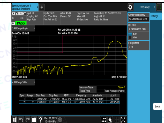
Band66-1.4MHz-16QAM-132665-1RB#0-PASS
