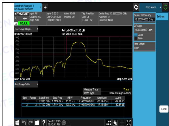
Band66-1.4MHz-16QAM-131979-6RB#0-PASS
