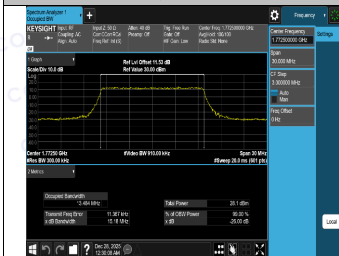
Band66-15MHz-16QAM-132322-27RB#0-PASS
