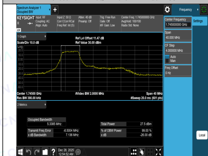
Band66-20MHz-16QAM-132322-27RB#0-PASS
