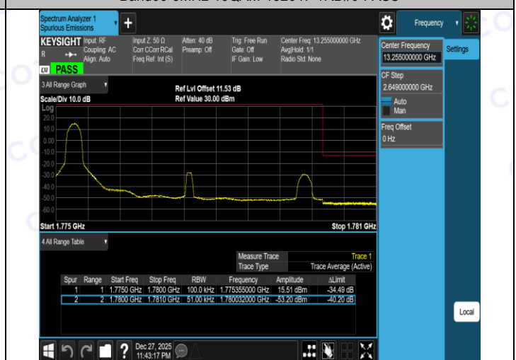
Band66-5MHz-16QAM-132647-25RB#0-PASS
