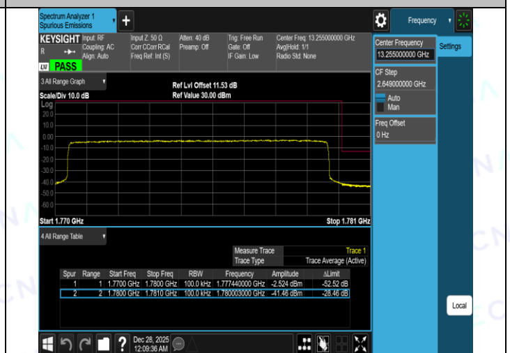
Band66-10MHz-16QAM-132022-1RB#49-PASS
