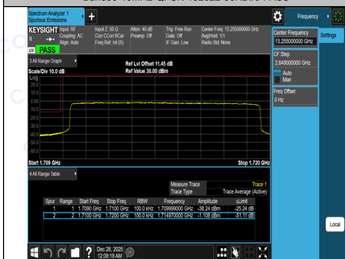
Band66-10MHz-QPSK-132622-1RB#49-PASS
