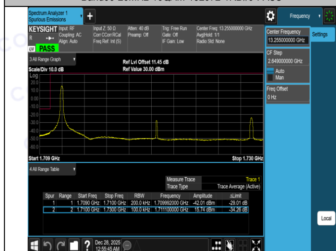
Band66-20MHz-16QAM-132572-1RB#0-PASS
