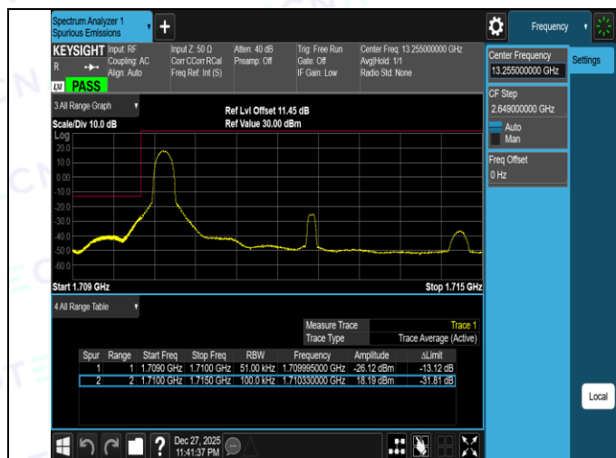
Band66-5MHz-QPSK-131997-25RB#0-PASS
