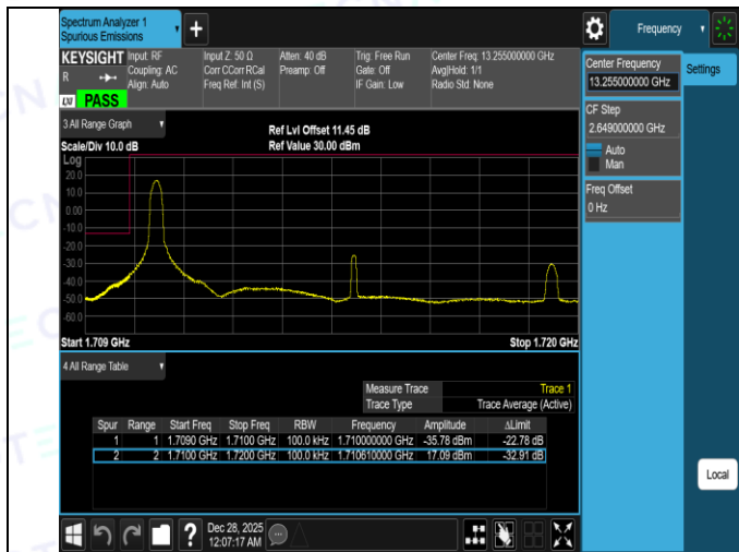
Band66-10MHz-QPSK-132022-50RB#0-PASS
