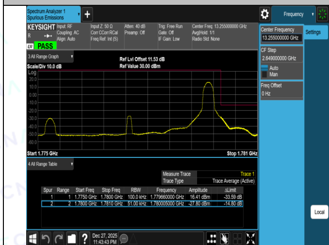
Band66-10MHz-QPSK-132022-1RB#0-PASS
