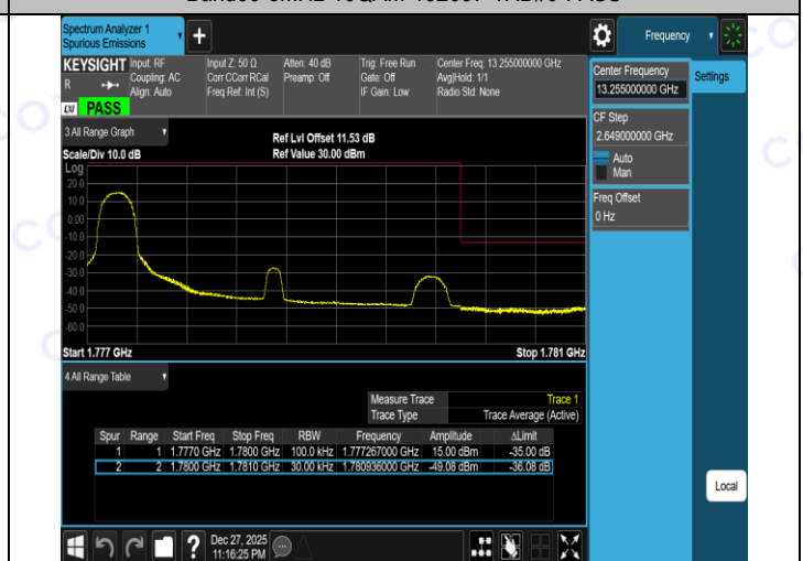
Band66-3MHz-16QAM-132657-15RB#0-PASS
