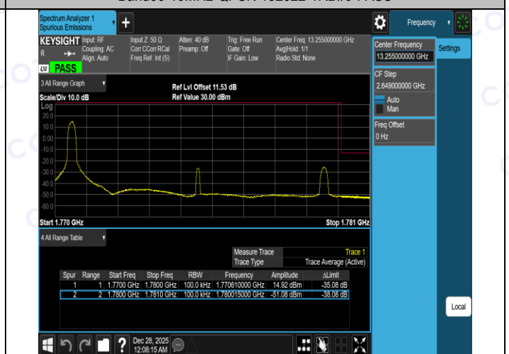
Band66-10MHz-QPSK-132622-50RB#0-PASS
