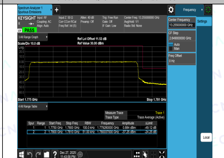
Band66-5MHz-16QAM-131997-1RB#24-PASS
