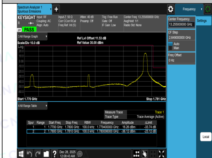
Band66-10MHz-16QAM-132022-1RB#0-PASS
