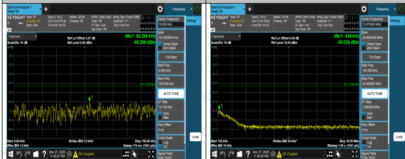
Band66-5MHz-QPSK-132647-1RB#0-30-1000-PASS
