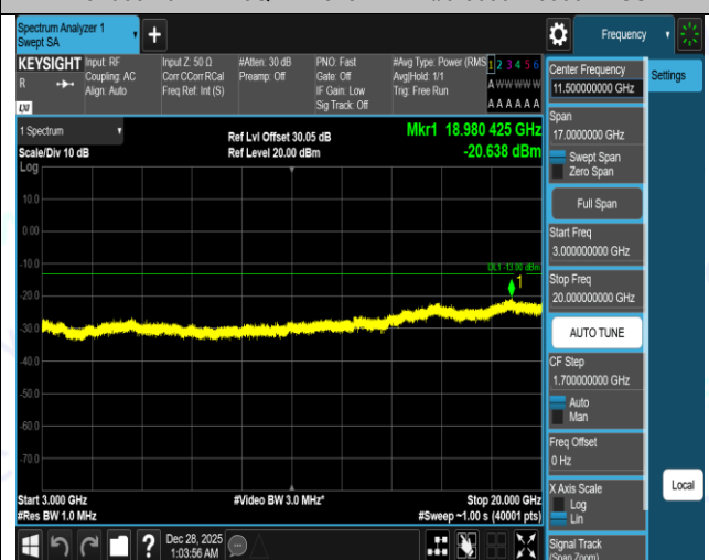
Band66-20MHz-16QAM-132572-1RB#0-3000~20000-PASS
