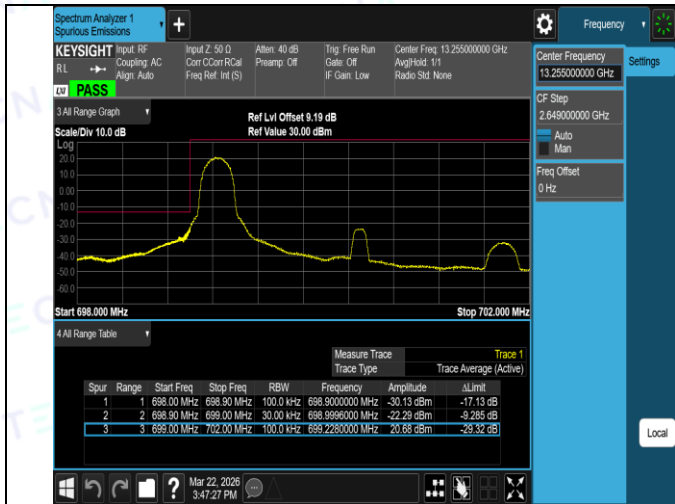
Band12-3MHz-QPSK-23025-15RB#0-PASS
