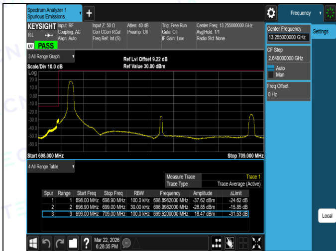
Band12-10MHz-QPSK-23060-50RB#0-PASS
