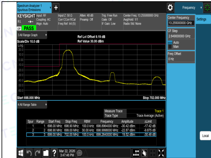
Band12-3MHz-16QAM-23025-15RB#0-PASS
