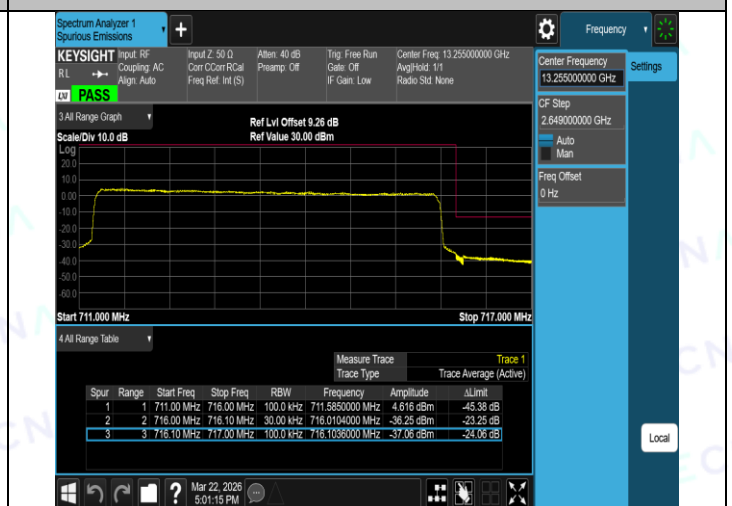
Band12-5MHz-16QAM-23035-1RB#24-PASS
