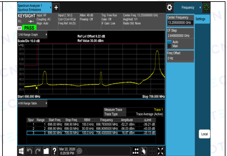
Band12-10MHz-16QAM-23130-1RB#49-PASS
