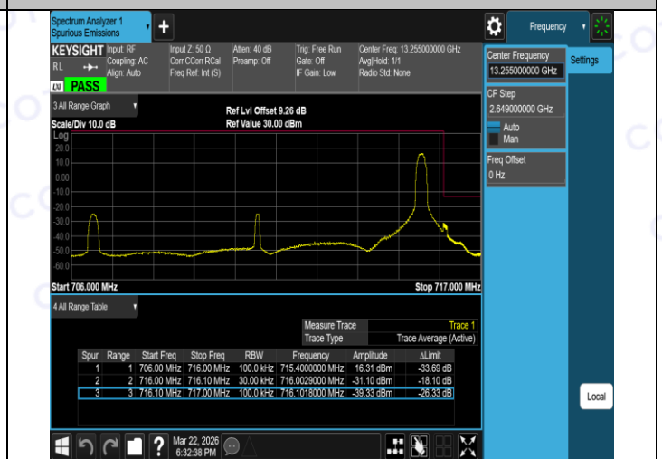
Band12-10MHz-16QAM-23130-1RB#49-PASS
