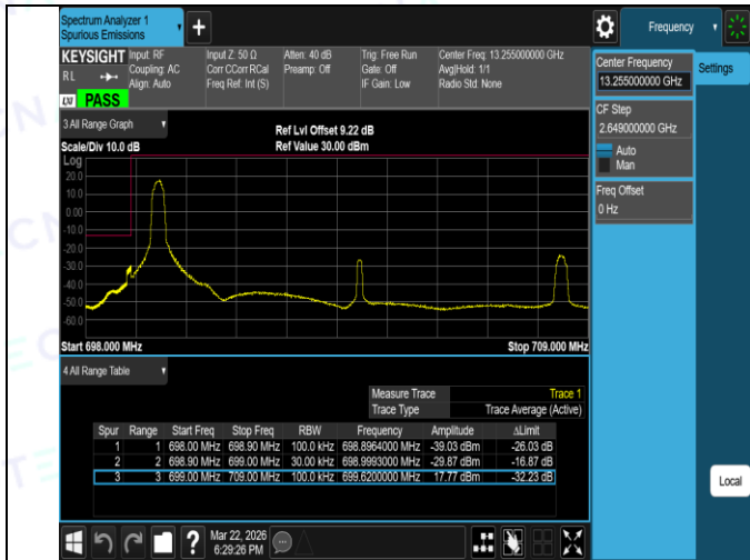
Band12-10MHz-16QAM-23130-1RB#0-PASS
