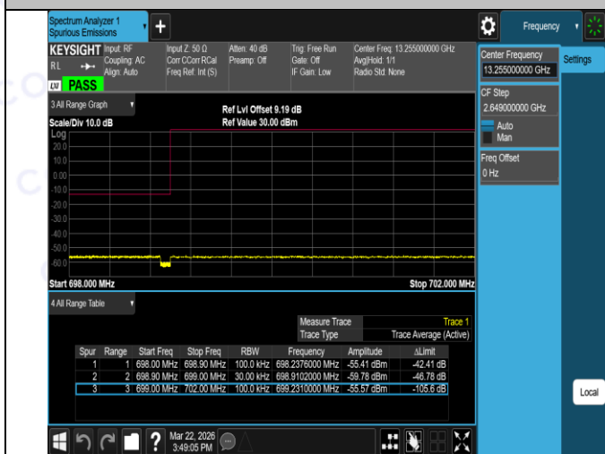
Band12-3MHz-16QAM-23165-1RB#14-PASS
