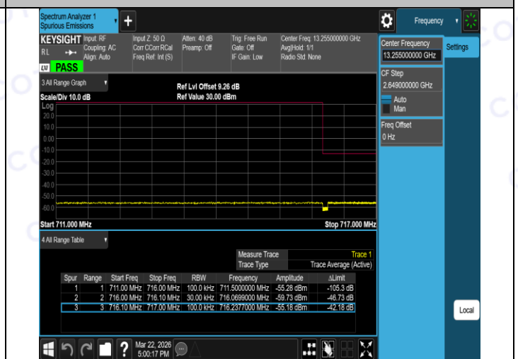
Band12-5MHz-16QAM-23155-25RB#0-PASS
