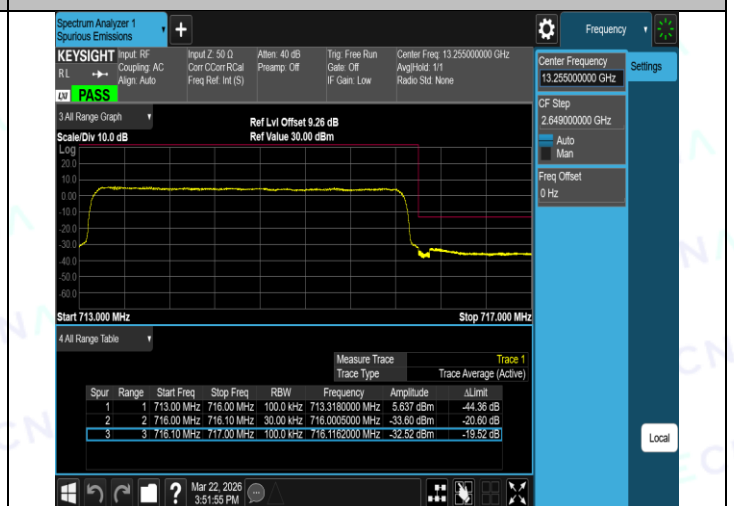
Band12-3MHz-16QAM-23025-1RB#14-PASS
