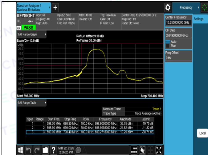
Band12-1.4MHz-16QAM-23017-6RB#0-PASS
