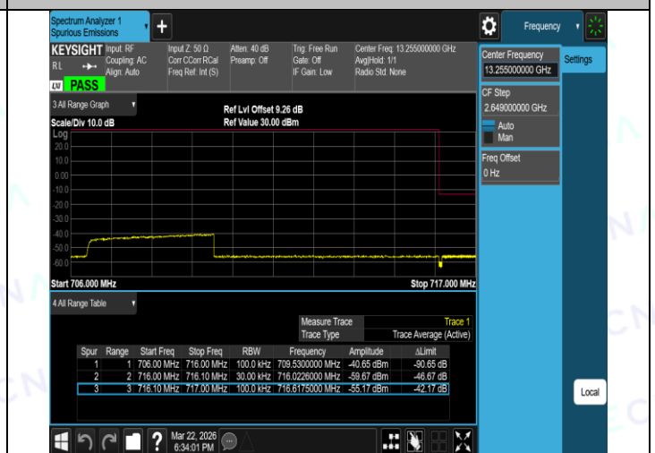
Band12-10MHz-16QAM-23060-1RB#49-PASS
