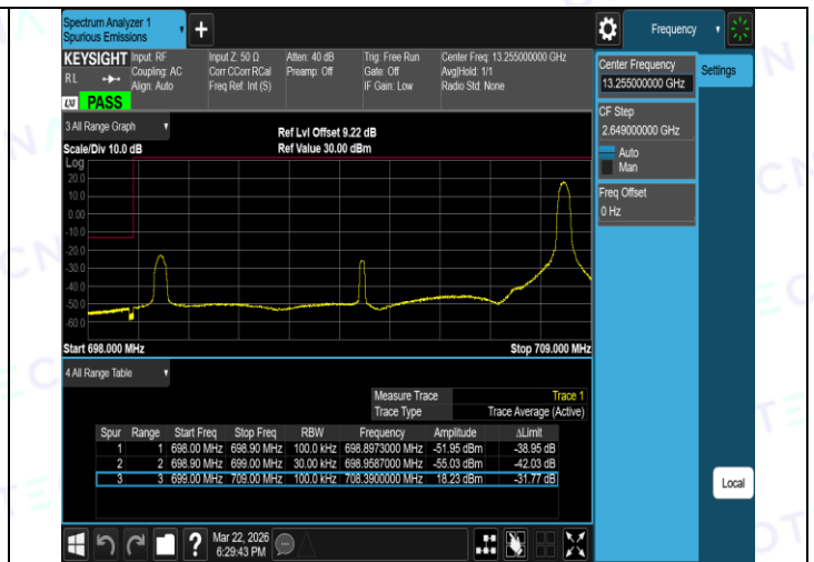
Band12-10MHz-QPSK-23130-1RB#0-PASS
