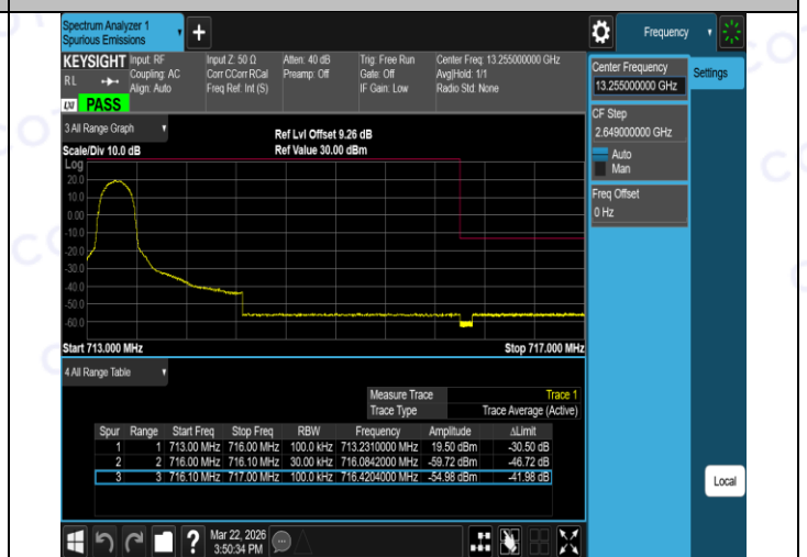
Band12-3MHz-QPSK-23165-15RB#0-PASS
