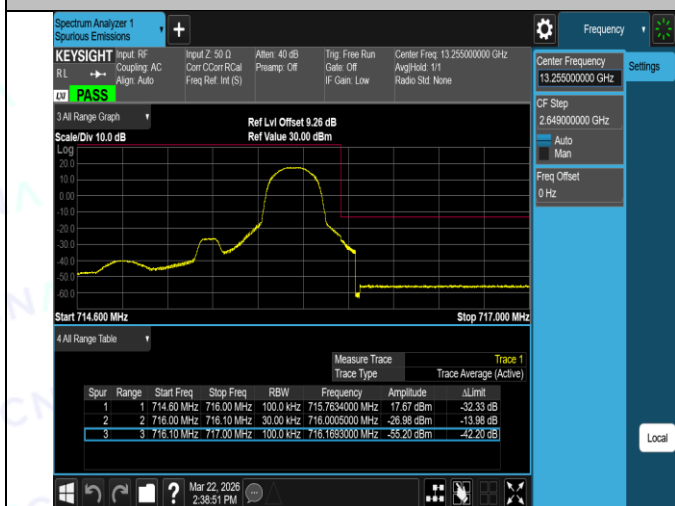
Band12-3MHz-QPSK-23025-1RB#0-PASS
