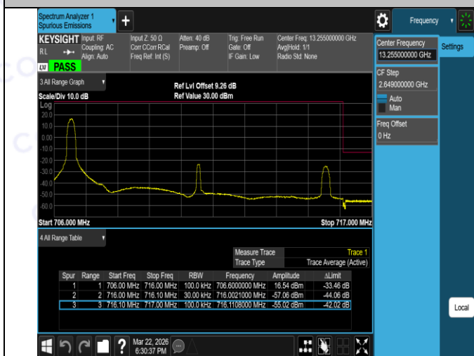
Band12-10MHz-16QAM-23130-1RB#0-PASS
