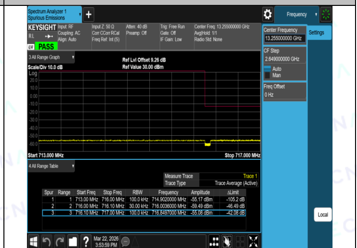
Band12-5MHz-QPSK-23035-1RB#24-PASS
