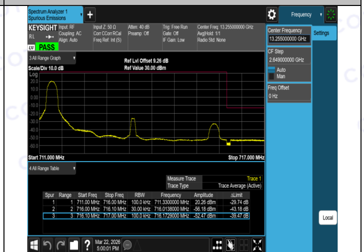
Band12-5MHz-QPSK-23155-25RB#0-PASS
