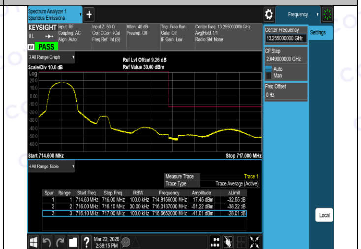
Band12-1.4MHz-16QAM-23173-6RB#0-PASS
