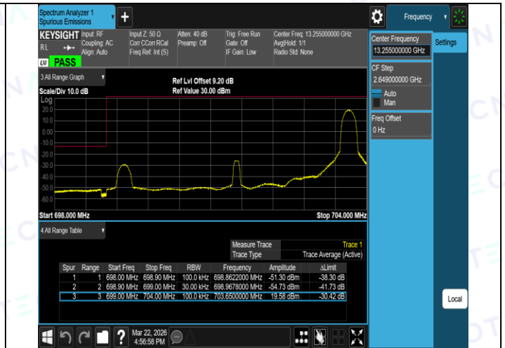
Band12-5MHz-QPSK-23155-1RB#0-PASS
