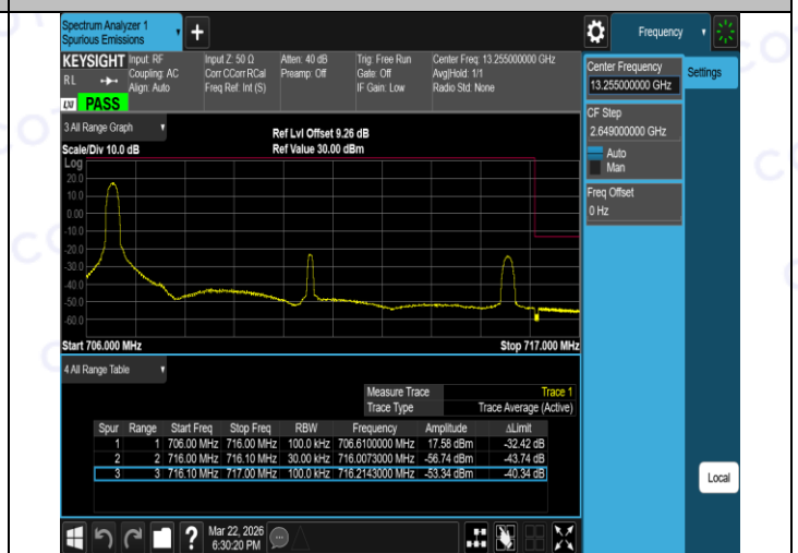
Band12-10MHz-QPSK-23130-50RB#0-PASS
