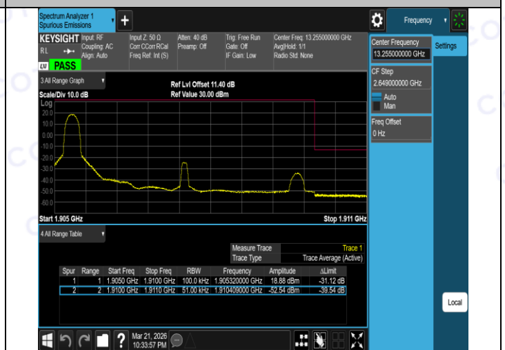
Band2-5MHz-QPSK-19175-25RB#0-PASS
