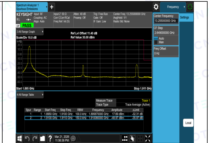
Band2-15MHz-QPSK-19125-75RB#0-PASS
