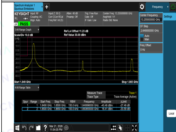
Band2-15MHz-QPSK-18675-75RB#0-PASS
