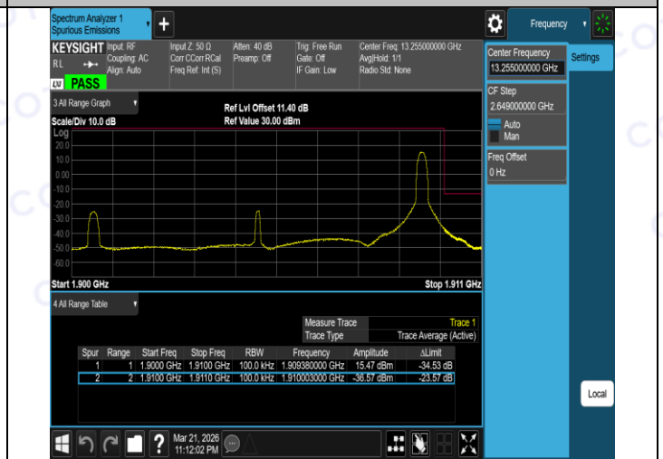
Band2-15MHz-QPSK-18675-1RB#74-PASS
