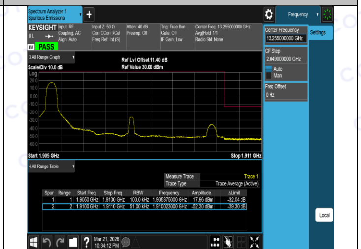
Band2-5MHz-16QAM-19175-25RB#0-PASS
