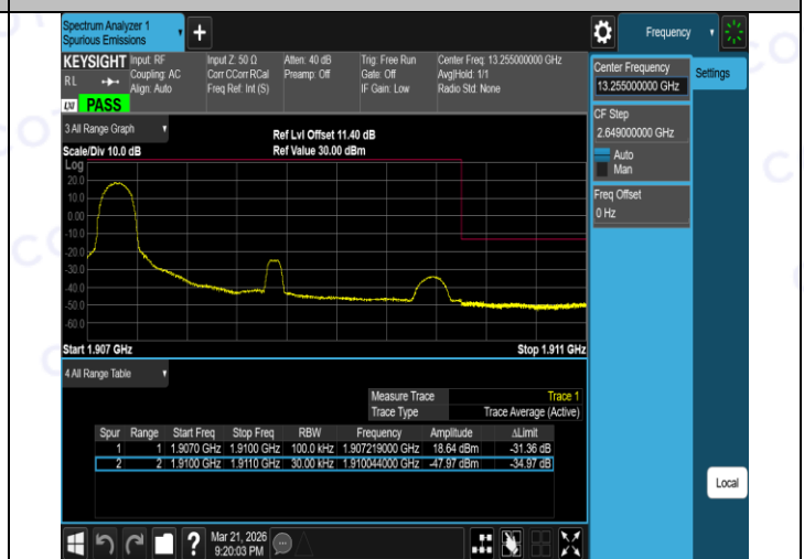
Band2-3MHz-QPSK-19185-15RB#0-PASS
