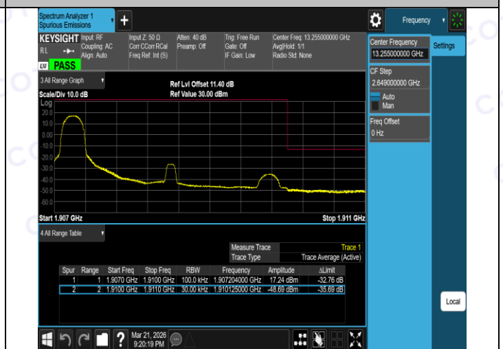
Band2-3MHz-16QAM-19185-15RB#0-PASS
