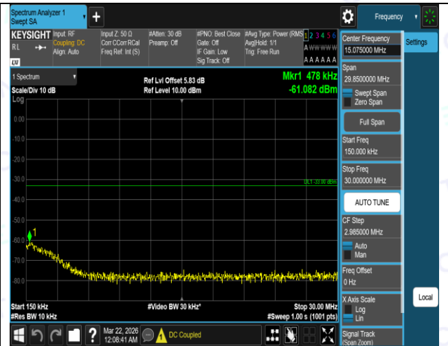
Band2-15MHz-QPSK-18675-1RB#0-1000~3000-PASS
