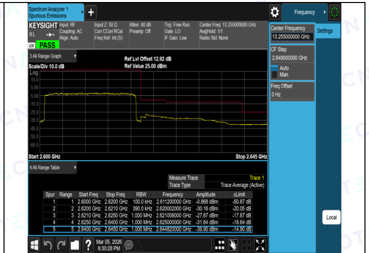
Band38-20MHz-16QAM-37850-1RB#99-PASS
