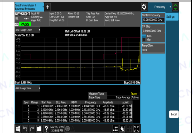
Band38-15MHz-QPSK-38175-1RB#0-PASS
