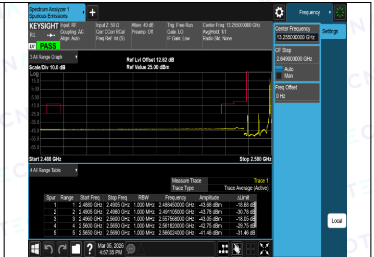
Band38-10MHz-16QAM-38200-1RB#49-PASS
