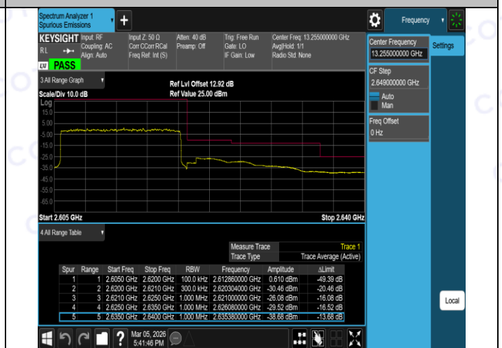
Band38-15MHz-16QAM-37825-1RB#74-PASS
