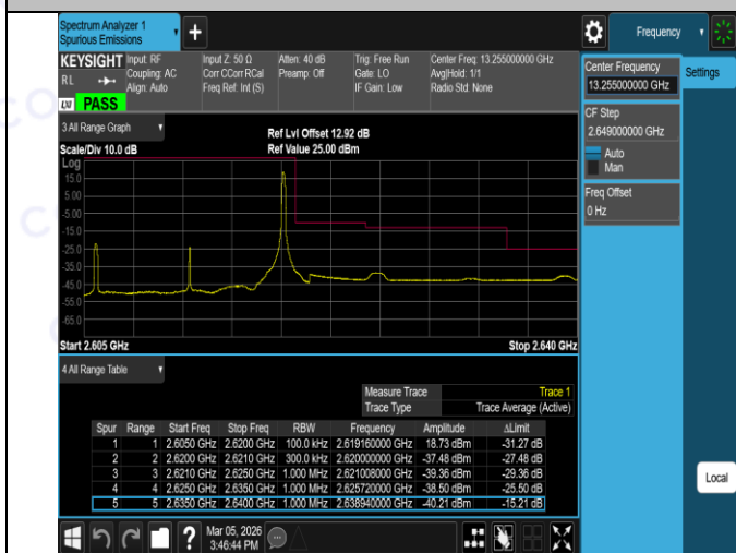
Band38-15MHz-16QAM-37825-1RB#0-PASS
