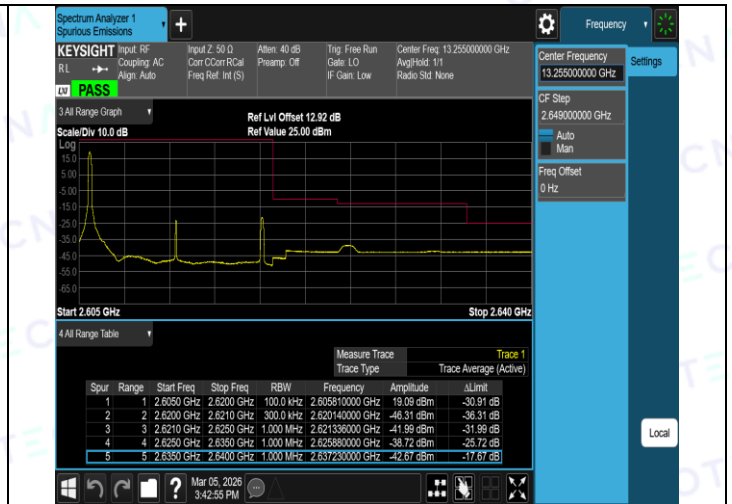
Band38-15MHz-QPSK-38175-75RB#0-PASS
