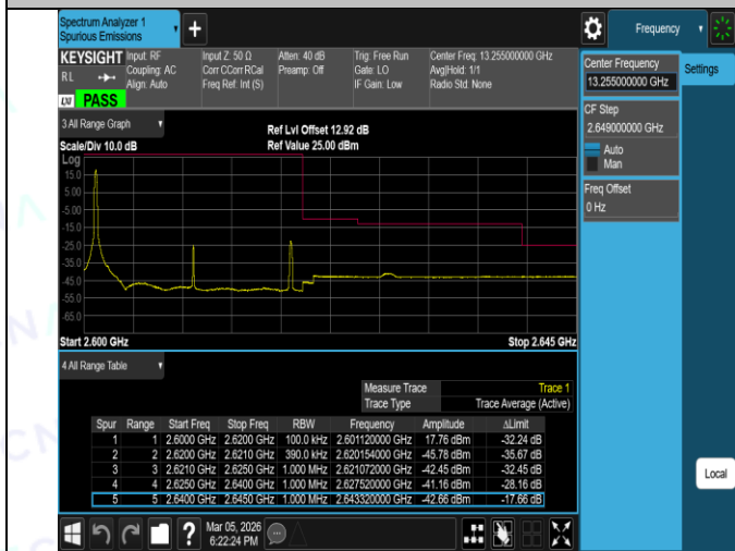
Band38-20MHz-16QAM-38150-1RB#0-PASS
