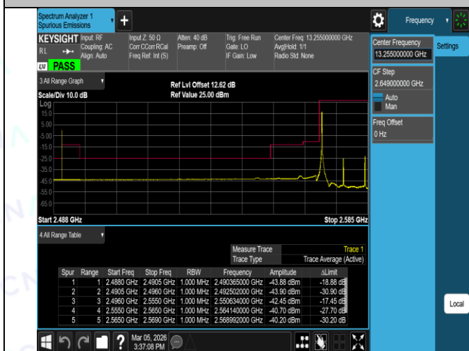
Band38-15MHz-16QAM-38175-1RB#0-PASS
