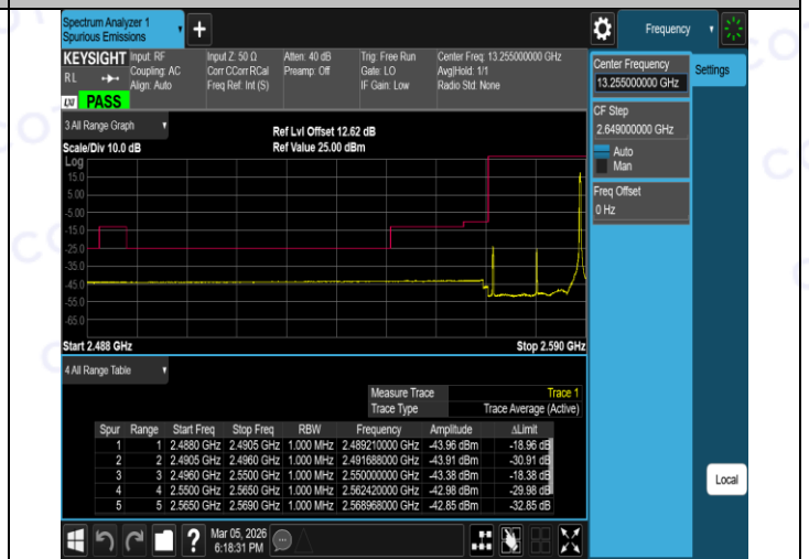
Band38-20MHz-16QAM-38150-1RB#99-PASS
