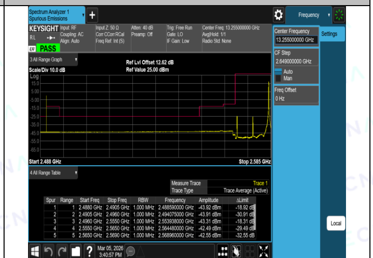
Band38-15MHz-16QAM-38175-1RB#74-PASS
