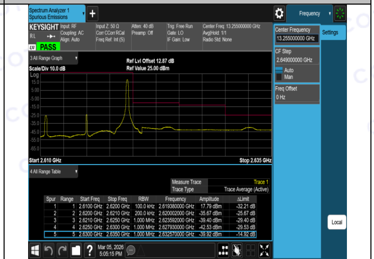
Band38-15MHz-QPSK-37825-1RB#74-PASS
