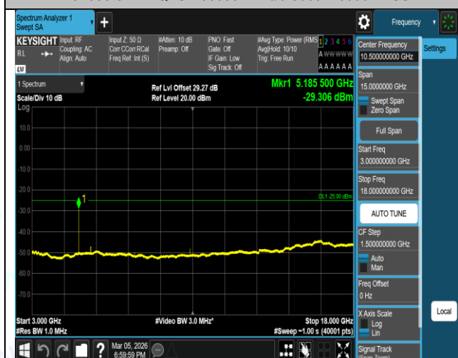
Band38-5MHz-QPSK-38225-1RB#0-0.009~0.15-PASS
