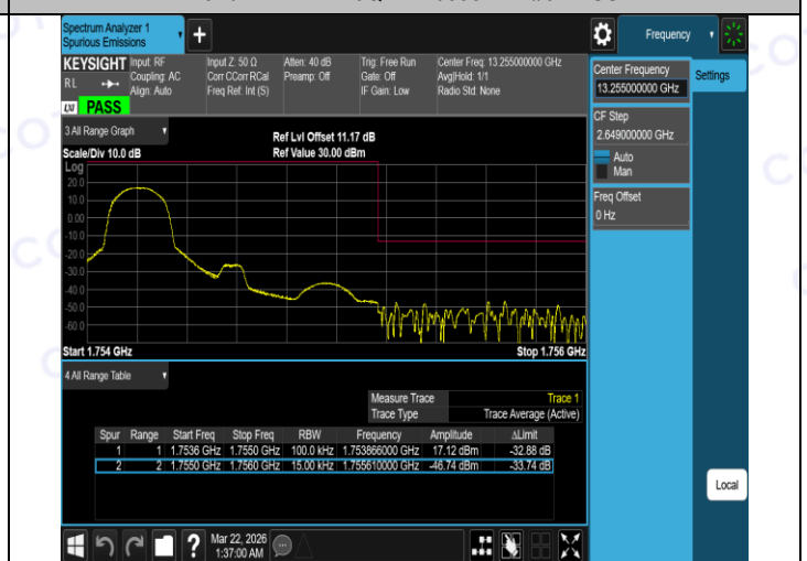
Band4-1.4MHz-16QAM-20393-6RB#0-PASS
