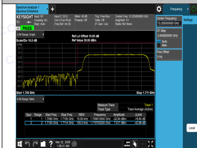
Band4-1.4MHz-16QAM-20393-1RB#5-PASS
