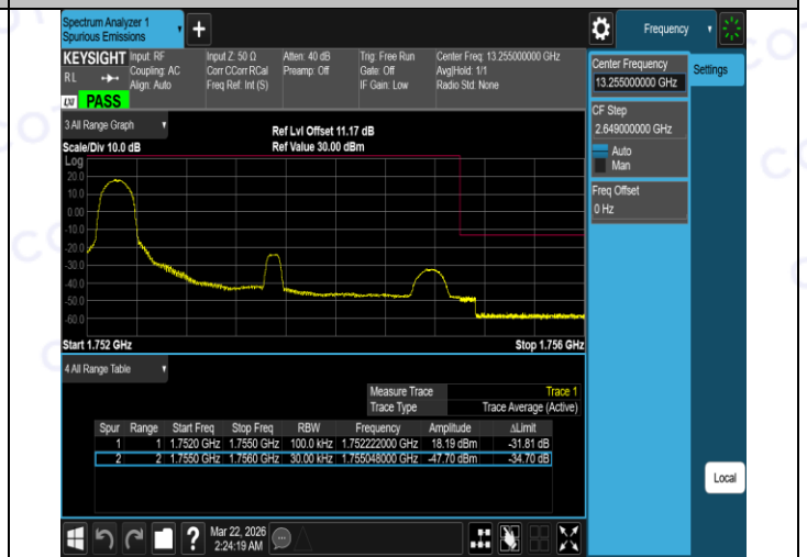
Band4-3MHz-QPSK-20385-15RB#0-PASS
