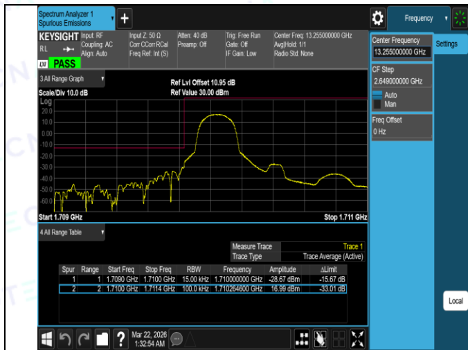
Band4-1.4MHz-16QAM-19957-6RB#0-PASS
