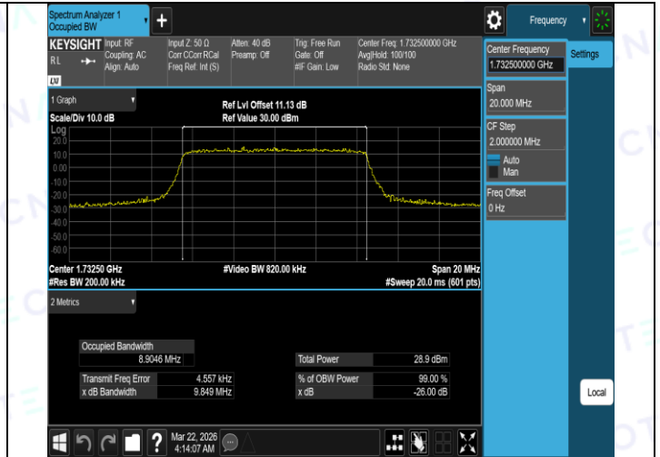
Band4-10MHz-16QAM-20000-27RB#0-PASS
