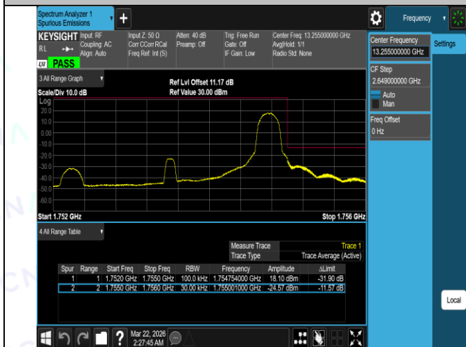
Band4-3MHz-16QAM-19965-1RB#0-PASS
