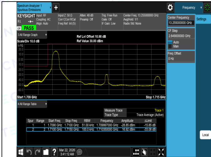
Band4-5MHz-16QAM-19975-25RB#0-PASS
