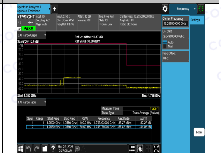
Band4-3MHz-16QAM-20385-15RB#0-PASS
