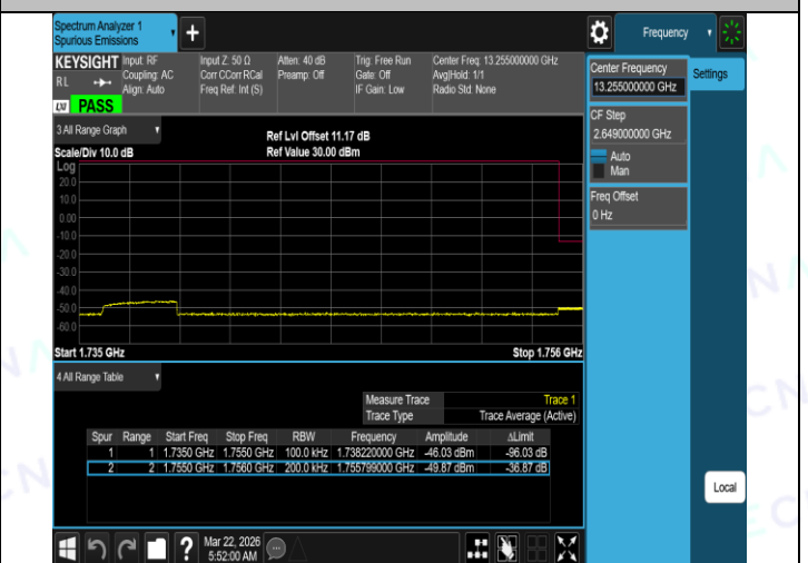
Band4-20MHz-QPSK-20300-100RB#0-PASS
