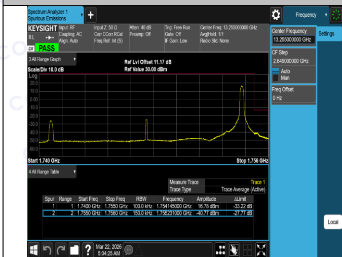
Band4-15MHz-16QAM-20025-1RB#0-PASS
