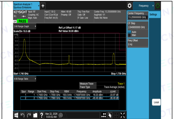
Band4-15MHz-QPSK-20325-75RB#0-PASS
