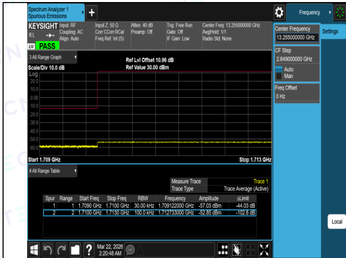
Band4-3MHz-16QAM-19965-15RB#0-PASS
