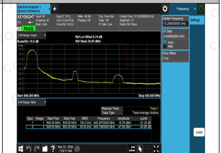
Band5-3MHz-16QAM-20635-15RB#0-PASS
