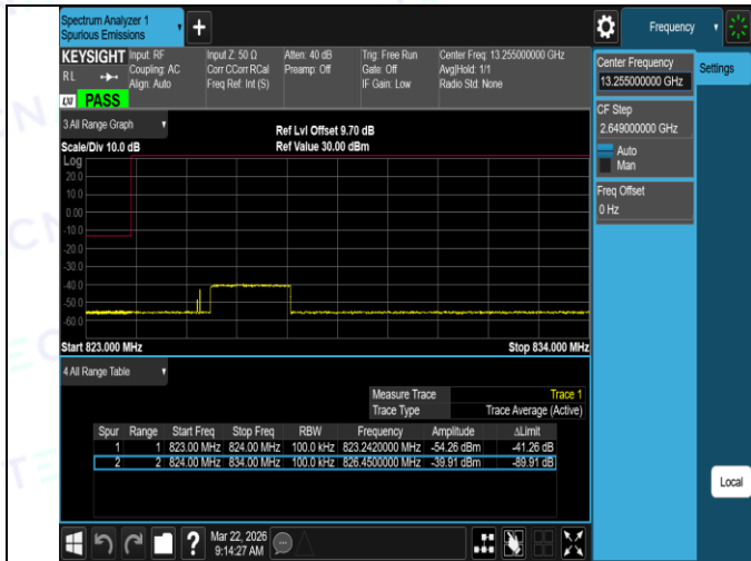
Band5-10MHz-QPSK-20450-50RB#0-PASS
