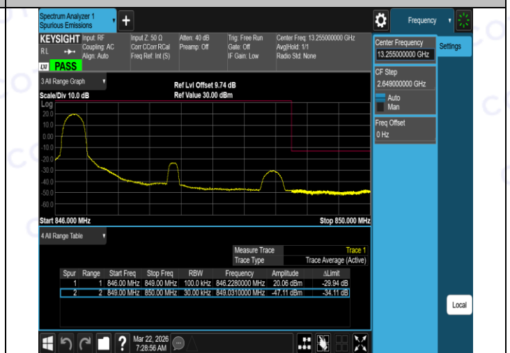
Band5-3MHz-QPSK-20635-15RB#0-PASS
