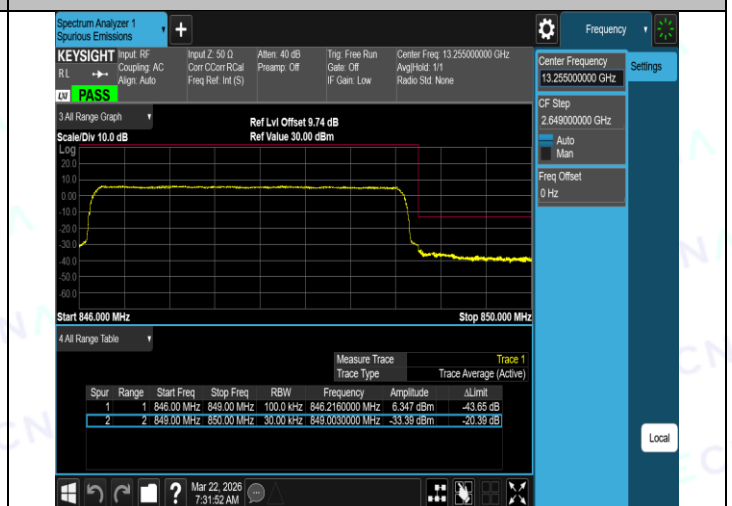
Band5-3MHz-16QAM-20415-1RB#14-PASS
