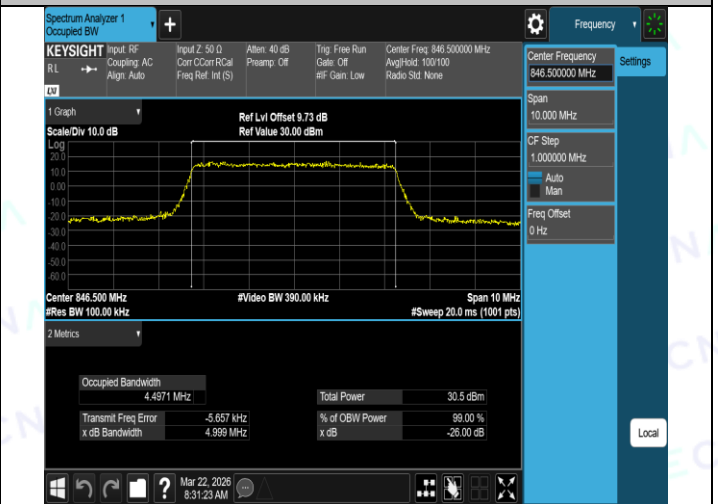
Band5-10MHz-QPSK-20525-50RB#0-PASS
