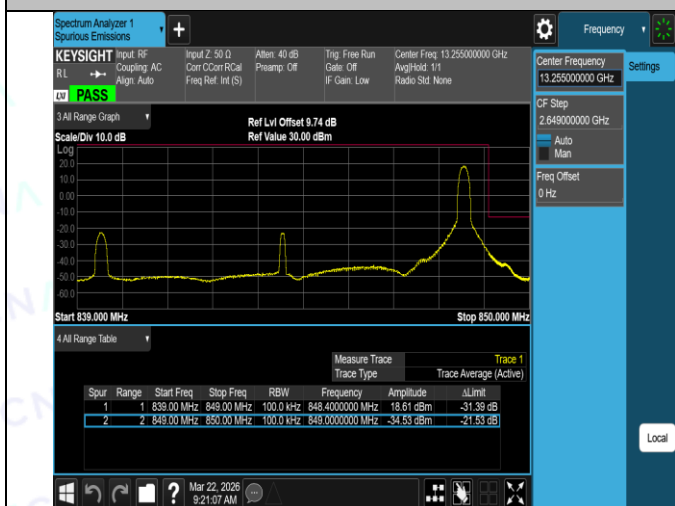
Band5-10MHz-16QAM-20450-1RB#0-PASS
