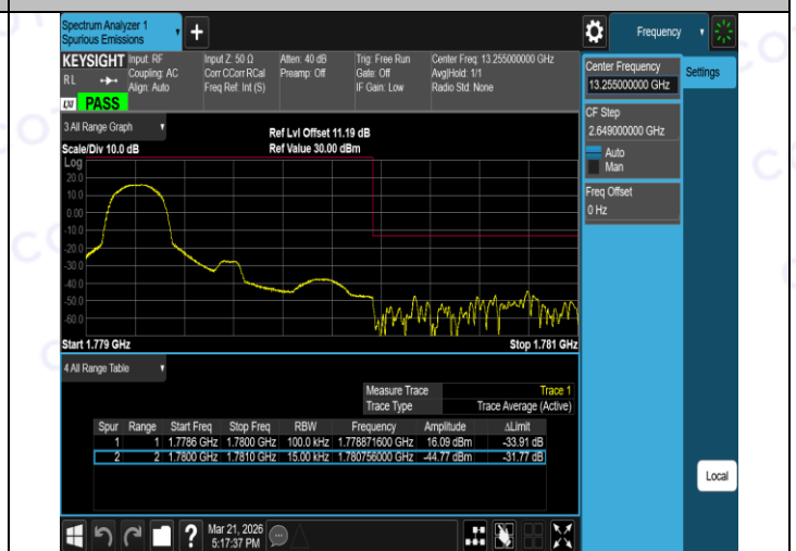
Band66-1.4MHz-16QAM-132665-6RB#0-PASS
