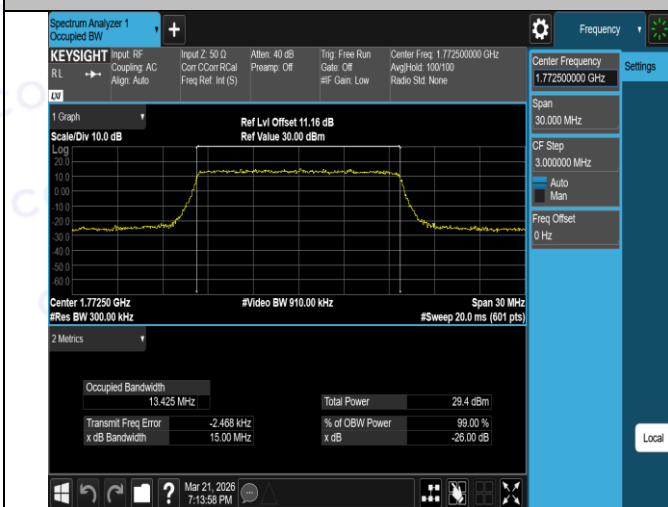
Band66-15MHz-16QAM-132322-27RB#0-PASS
