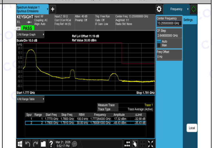
Band66-3MHz-QPSK-132657-15RB#0-PASS
