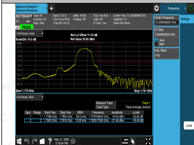
Band66-3MHz-QPSK-131987-1RB#0-PASS
