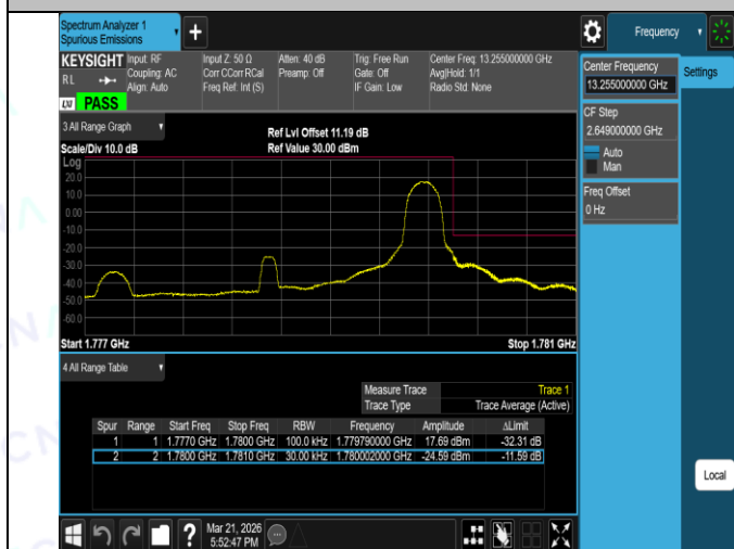
Band66-3MHz-16QAM-131987-1RB#0-PASS
