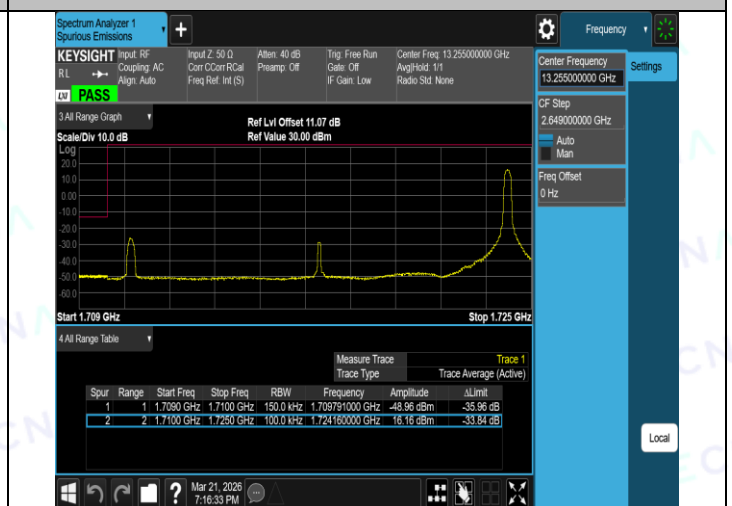
Band66-15MHz-16QAM-132597-1RB#74-PASS
