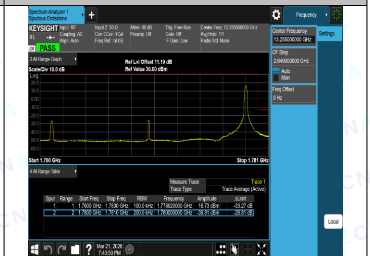
Band66-20MHz-16QAM-132572-1RB#99-PASS
