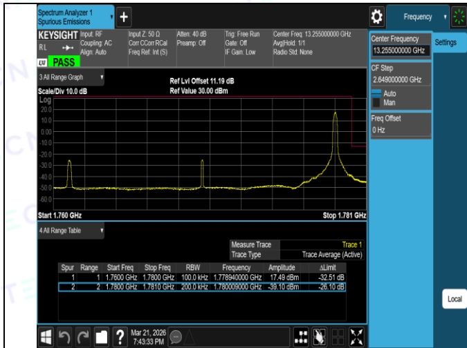
Band66-20MHz-16QAM-132072-1RB#0-PASS
