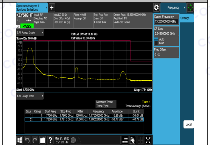
Band66-5MHz-16QAM-132647-25RB#0-PASS
