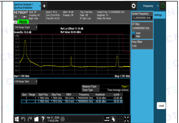
Band66-15MHz-QPSK-132597-75RB#0-PASS
