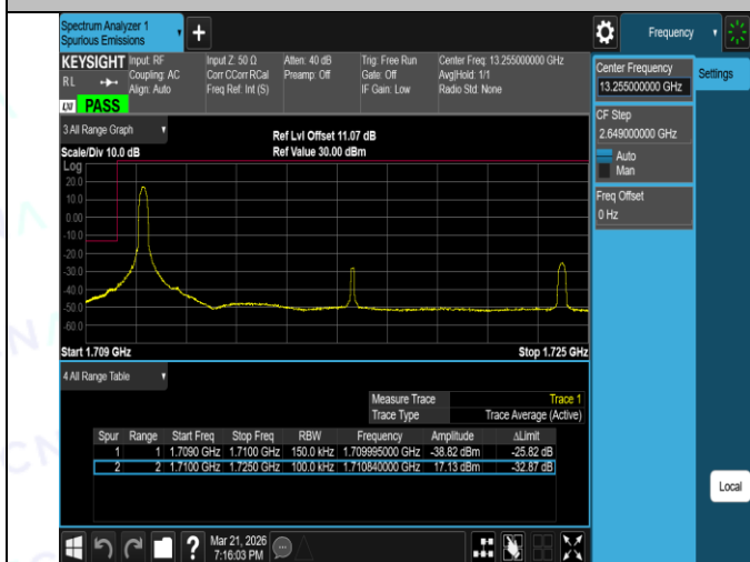
Band66-15MHz-16QAM-132597-1RB#0-PASS
