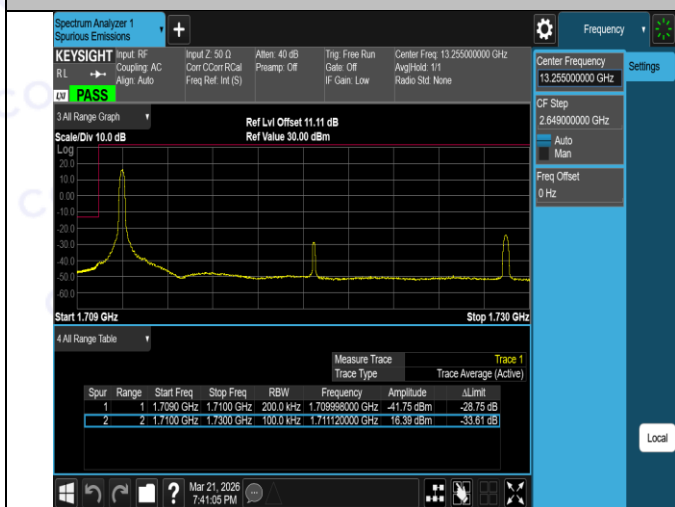
Band66-20MHz-QPSK-132072-100RB#0-PASS
