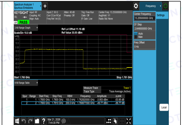
Band66-20MHz-16QAM-132072-1RB#99-PASS
