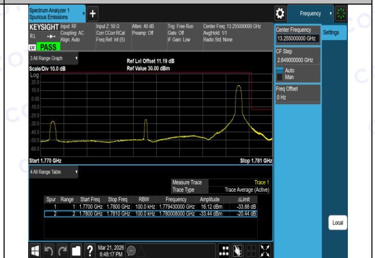
Band66-15MHz-QPSK-132047-1RB#74-PASS
