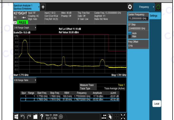
Band66-5MHz-QPSK-132647-25RB#0-PASS
