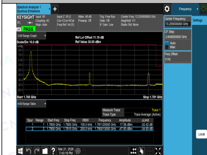
Band66-20MHz-16QAM-132572-1RB#0-PASS
