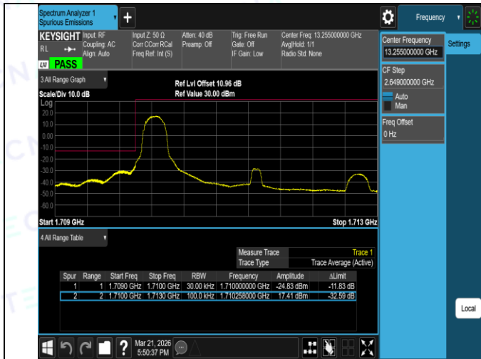
Band66-3MHz-16QAM-131987-15RB#0-PASS
