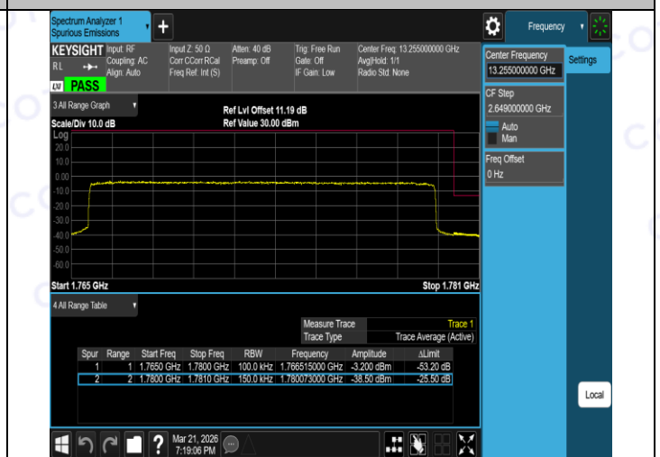
Band66-15MHz-16QAM-132047-1RB#74-PASS
