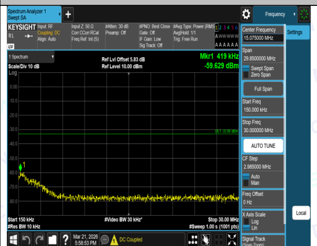
Band66-3MHz-QPSK-132657-1RB#0-1000~3000-PASS
