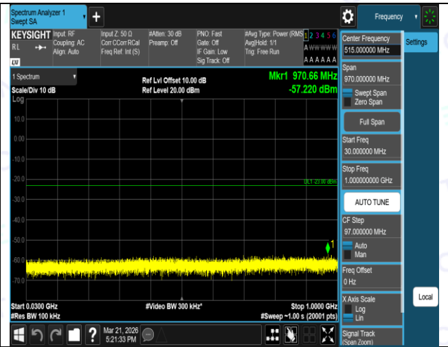
Band66-1.4MHz-QPSK-132322-1RB#0-3000~20000-PASS
