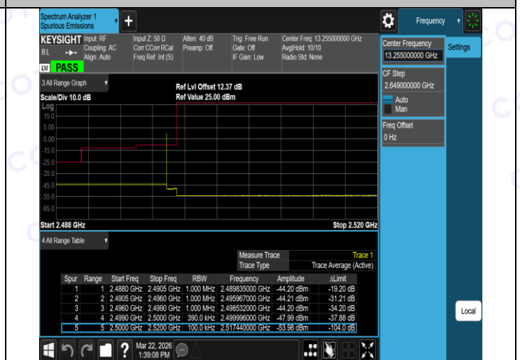
Band7-20MHz-QPSK-20850-100RB#99-PASS
