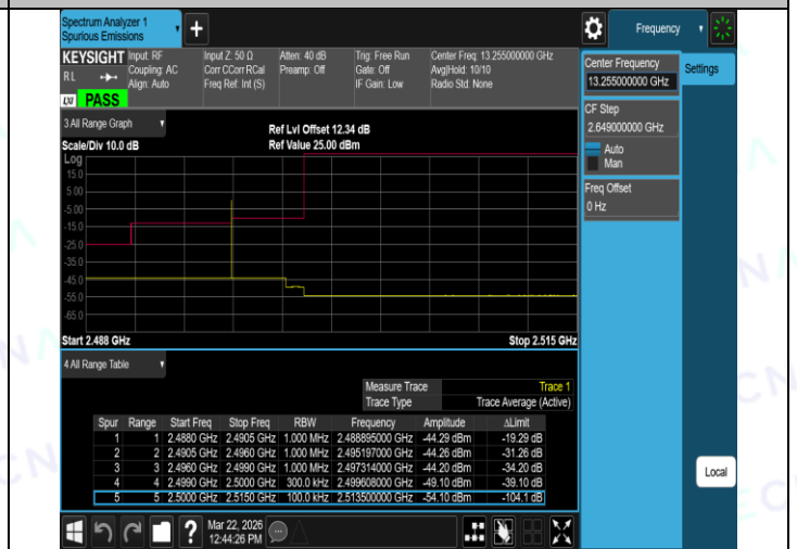
Band7-15MHz-16QAM-21375-1RB#74-PASS
