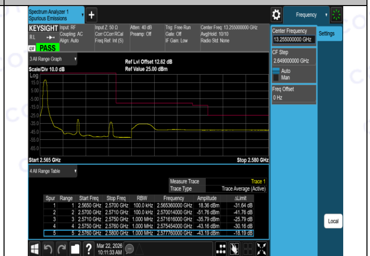
Band7-5MHz-16QAM-21425-25RB#0-PASS
