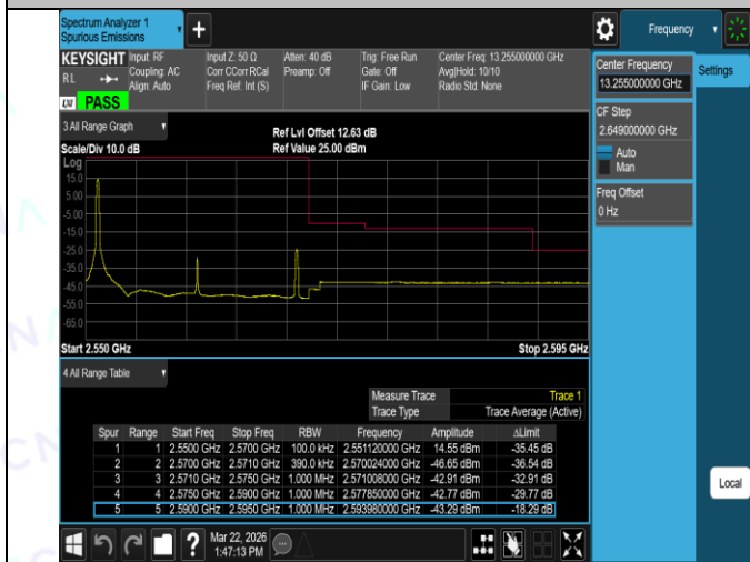
Band7-20MHz-16QAM-21350-1RB#0-PASS
