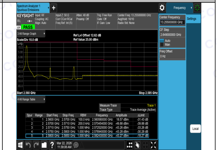
Band7-10MHz-QPSK-21400-50RB#0-PASS
