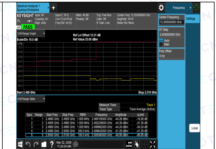
Band7-10MHz-16QAM-21400-1RB#49-PASS
