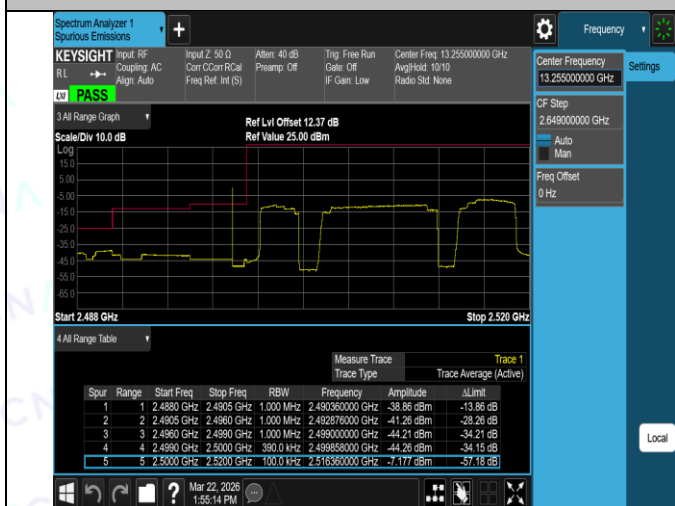
Band7-20MHz-QPSK-21350-1RB#0-PASS
