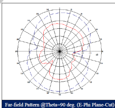
Far-field Pattern @Theta=90 deg. (E-Phi Plane-Cut)
