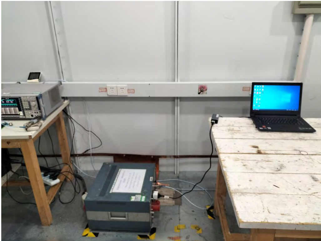
Photo of Conducted Emission Measurement
