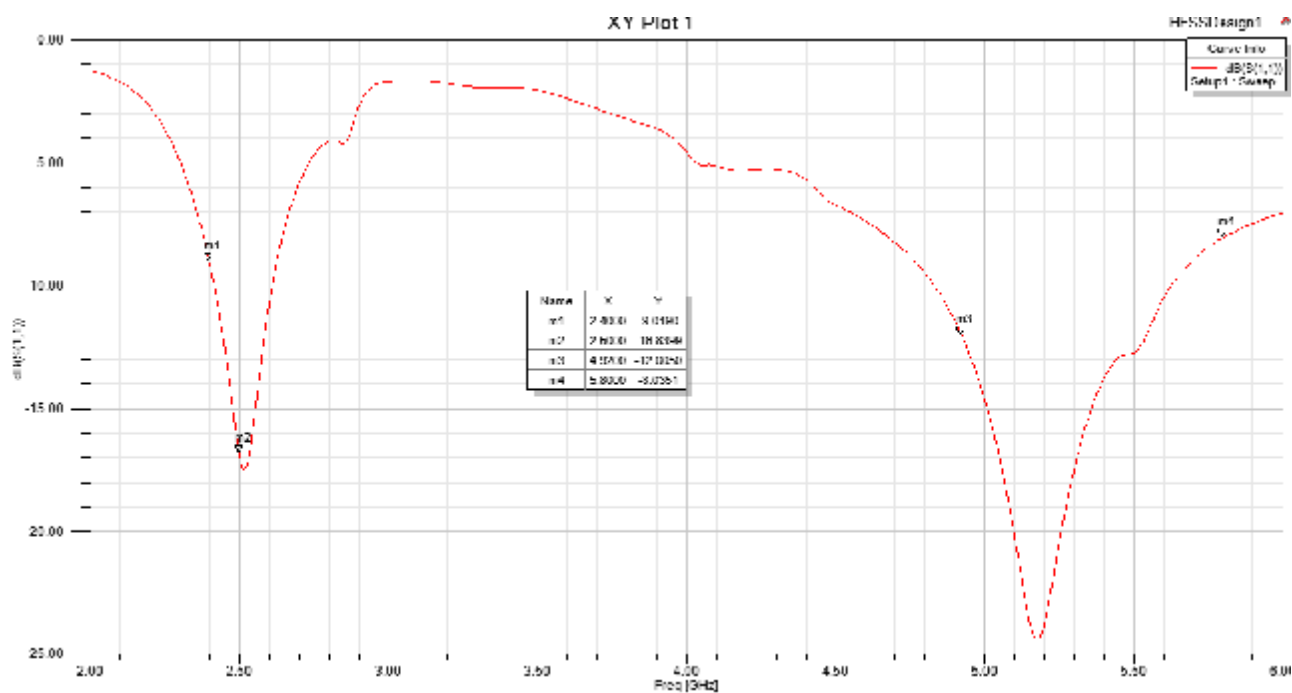
Figure 2 Left PIFA antenna return loss
