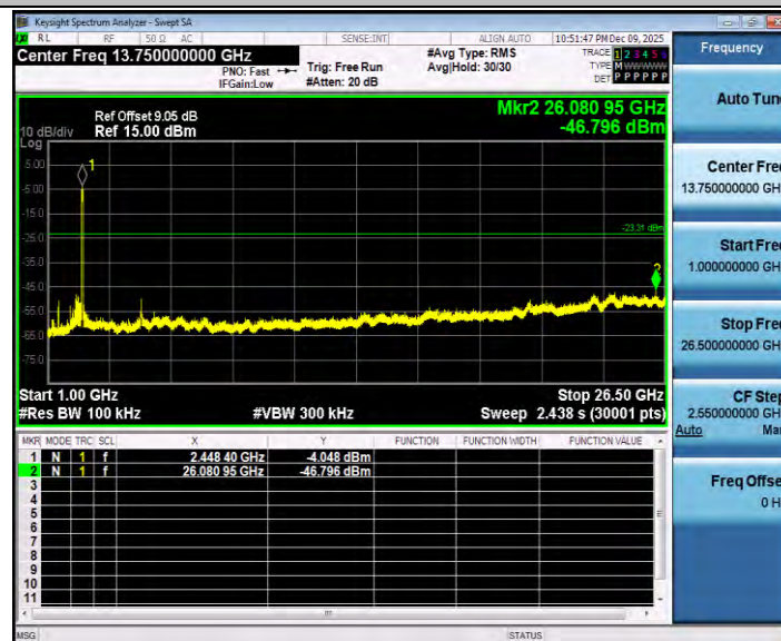
11AX40SISO_Ant1_2437_1000~26500
