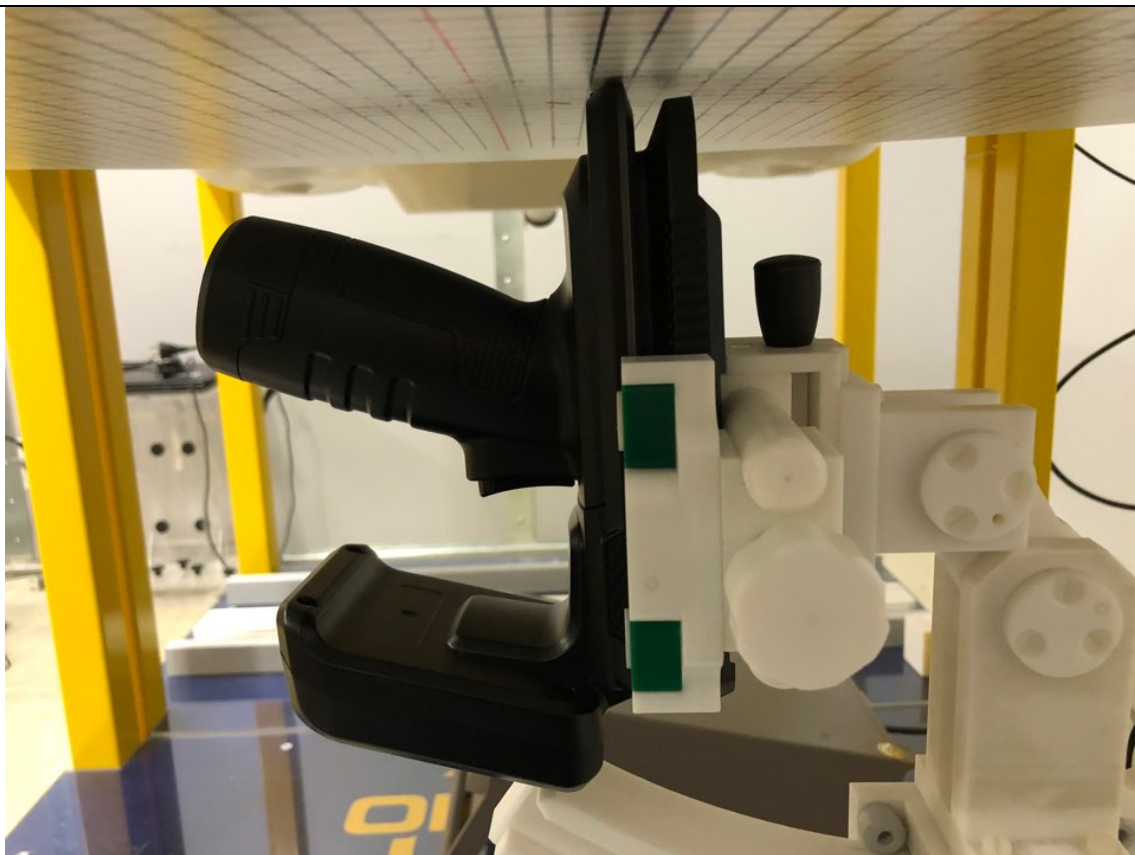
Rear (0 mm)
