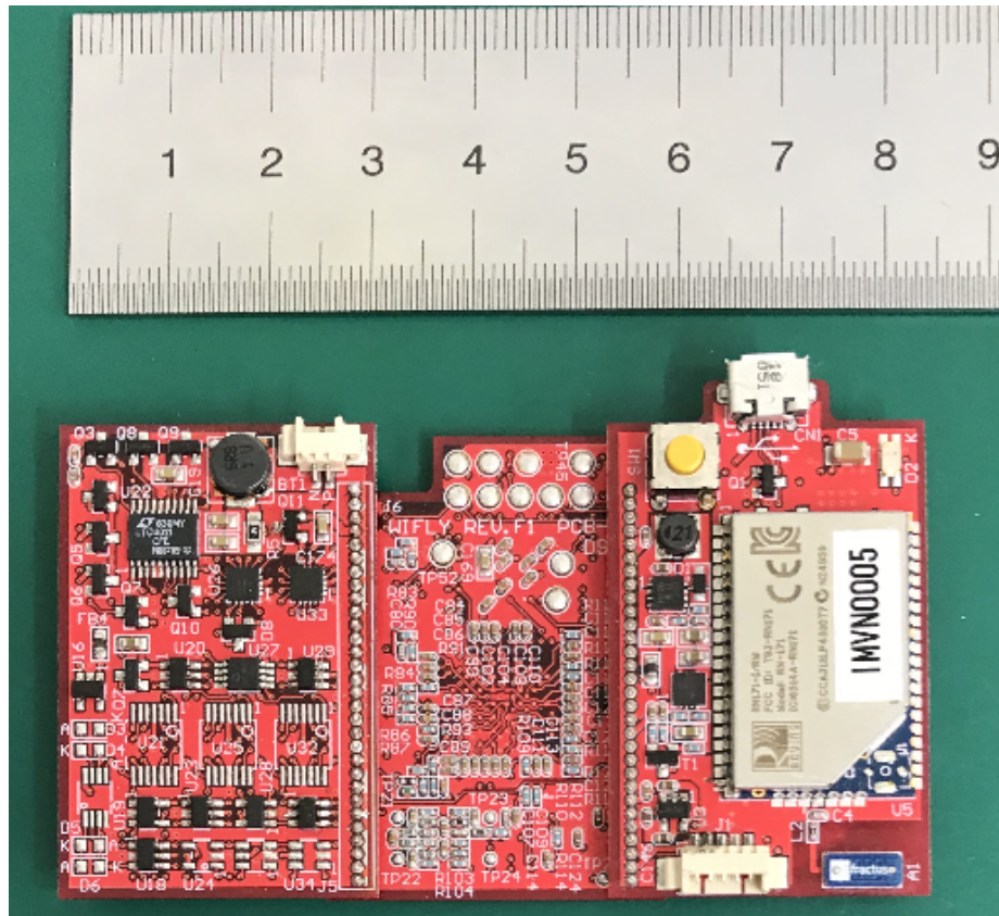
3 rd Board
