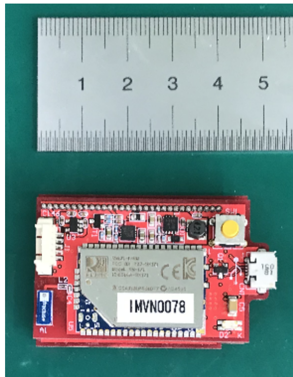
PCB_1: Top
