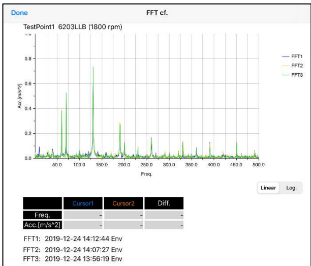
Figure 4.40 FFT cf.
