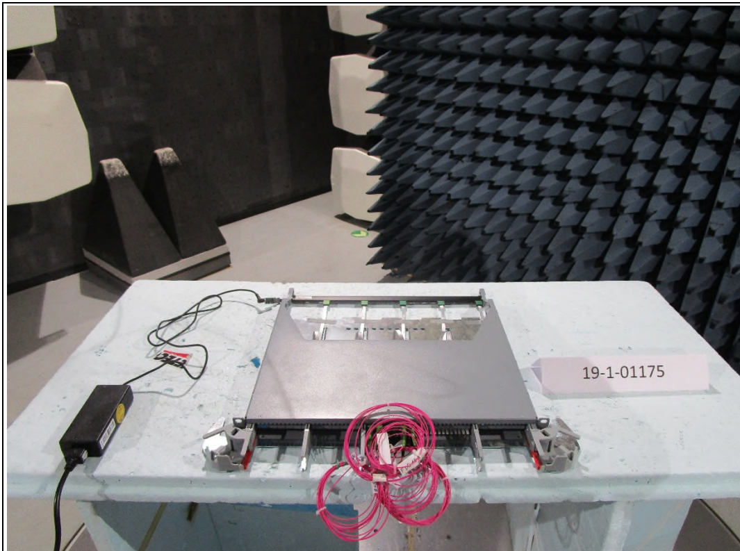
Photograph 3: Radiated measurements test set-up close up view
