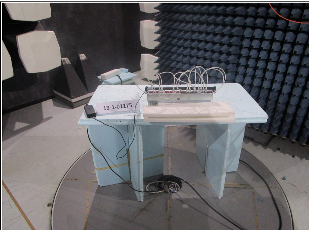
Photograph 4: Test set-up
