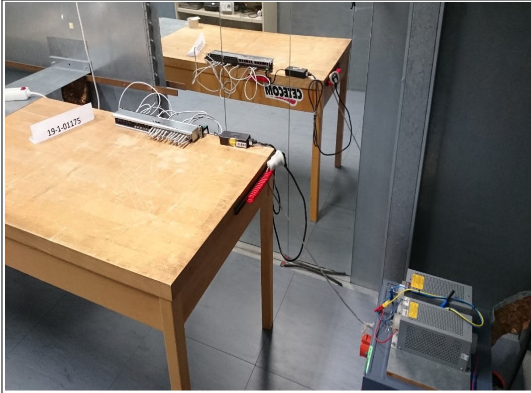
Photograph 1: Conducted measurements test set-up
