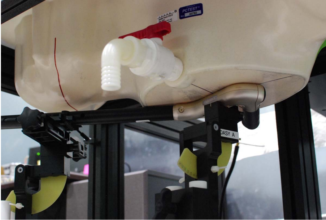
SAR Test Setup Photo 6 – Body, Left Side at 0mm
