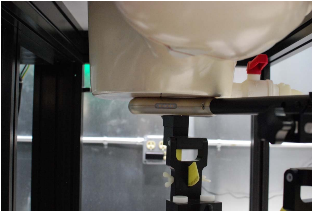
SAR Test Setup Photo 5 – Body, Right Side at 0mm
