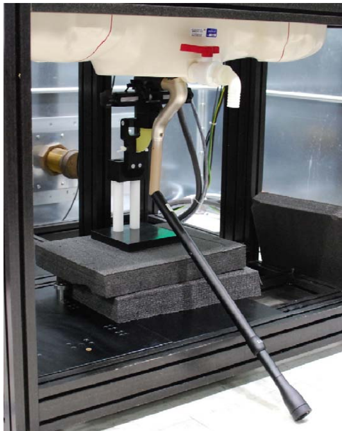
SAR Test Setup Photo 3 – Body, Top Side at 0mm
