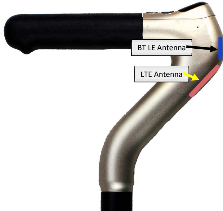
Figure G-1 DUT Antenna Locations
