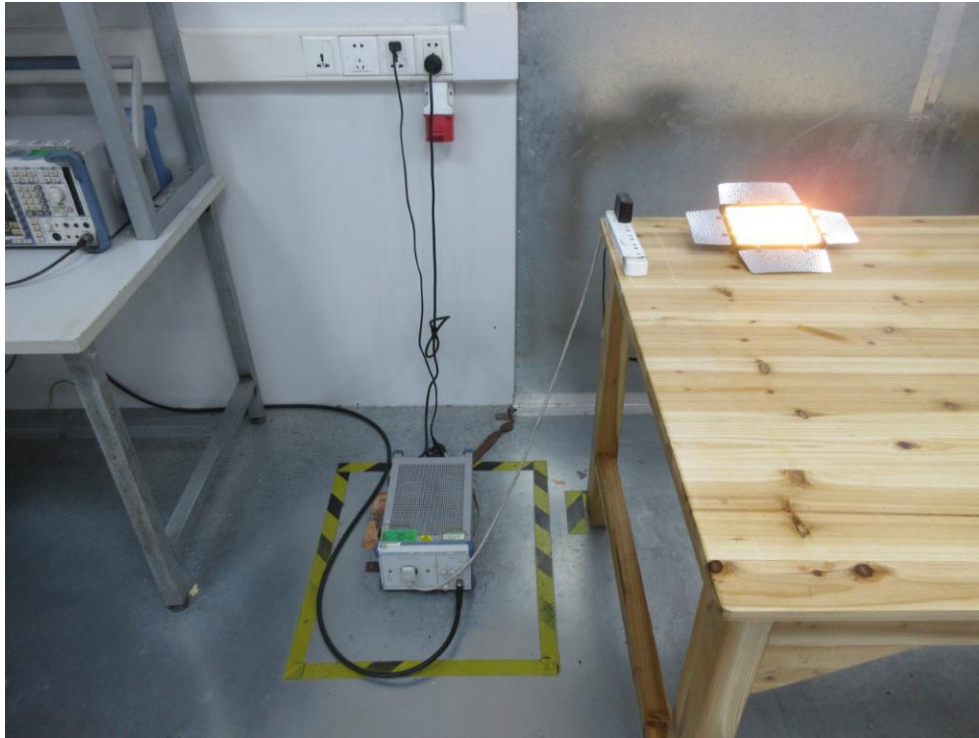
FCC ID: 2AVFB- SL-240E Photo of Conducted Emission Test
