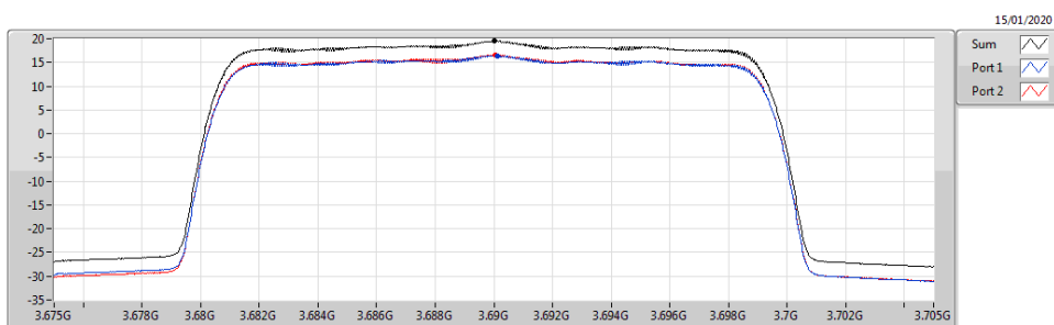
Band 48_LTE_20MHz_Nss1,16QAM_2TX 3690MHz_16QAM_RB 100,#RB 0
