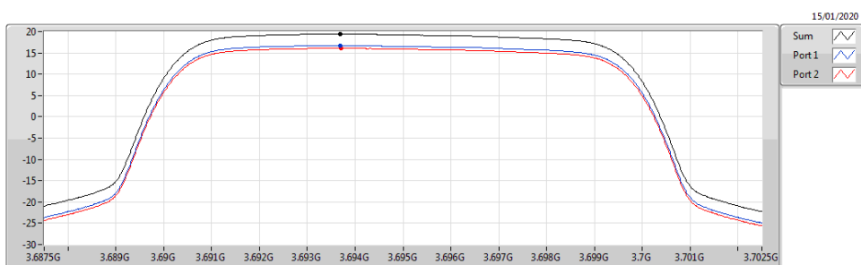
Band 48_LTE_10MHz_Nss1,64QAM_2TX 3695MHz_64QAM_RB 50,#RB 0
