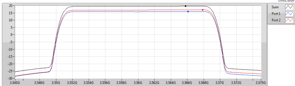
Band 48_LTE_20MHz_Nss1,64QAM_2TX 3560MHz_64QAM_RB 100,#RB 0
