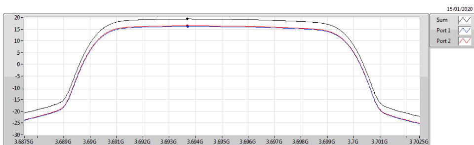
Band 48_LTE_10MHz_Nss1,QPSK_2TX 3695MHz_QPSK_RB 50,#RB 0
