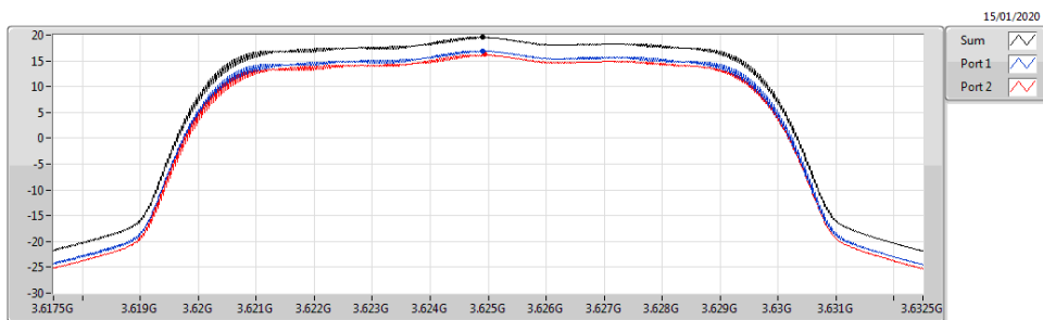
Band 48_LTE_10MHz_Nss1,16QAM_2TX 3625MHz_16QAM_RB 50,#RB 0
