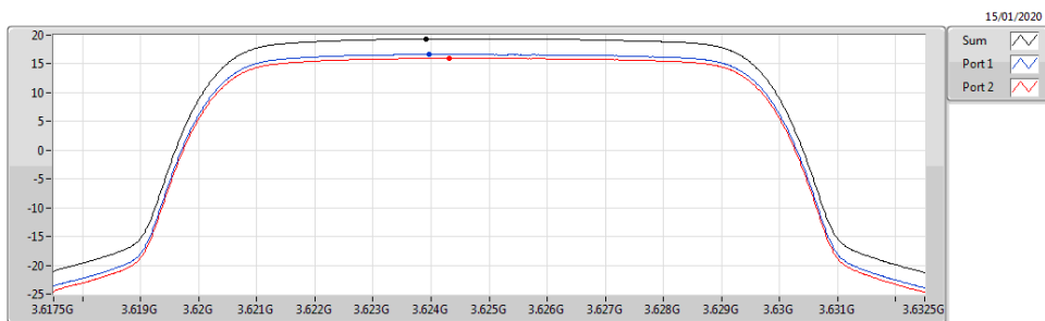
Band 48_LTE_10MHz_Nss1,64QAM_2TX 3625MHz_64QAM_RB 50,#RB 0
