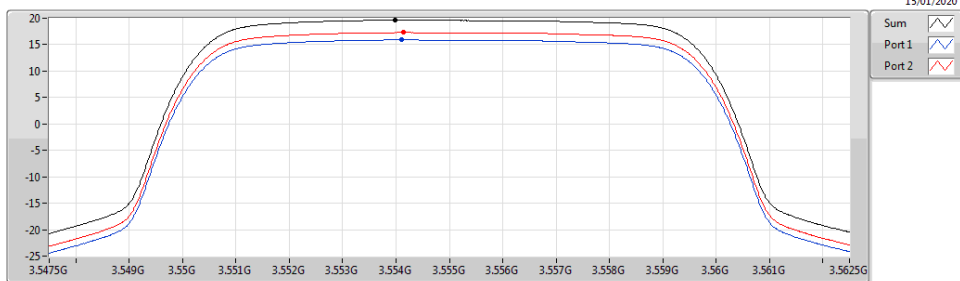
Band 48_LTE_10MHz_Nss1,64QAM_2TX 3555MHz_64QAM_RB 50,#RB 0
