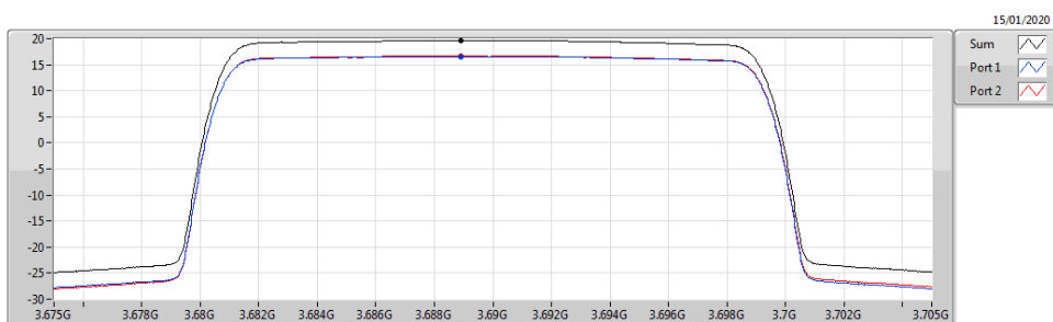
Band 48_LTE_20MHz_Nss1,64QAM_2TX 3690MHz_64QAM_RB 100,#RB 0
