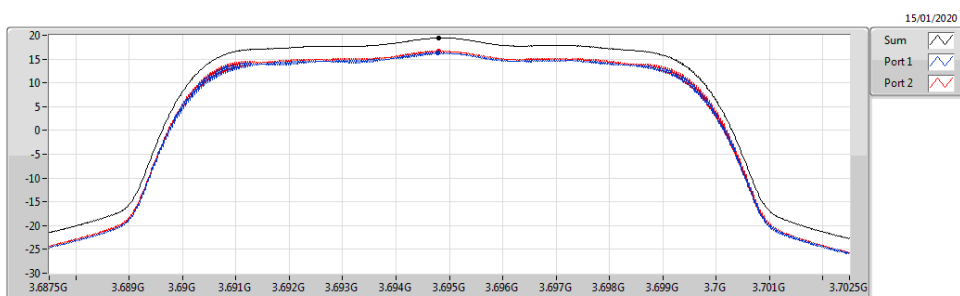
Band 48_LTE_10MHz_Nss1,16QAM_2TX 3695MHz_16QAM_RB 50,#RB 0
