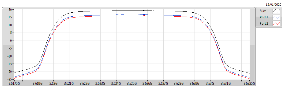
Band 48_LTE_10MHz_Nss1,QPSK_2TX 3625MHz_QPSK_RB 50,#RB 0
