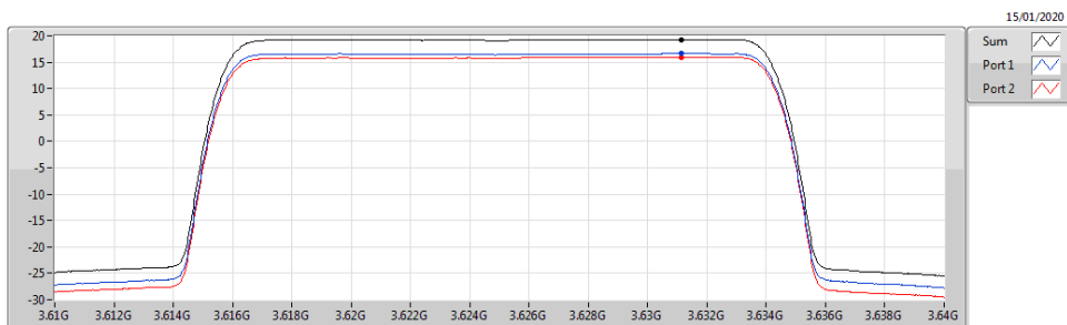
Band 48_LTE_20MHz_Nss1,64QAM_2TX 3625MHz_64QAM_RB 100,#RB 0
