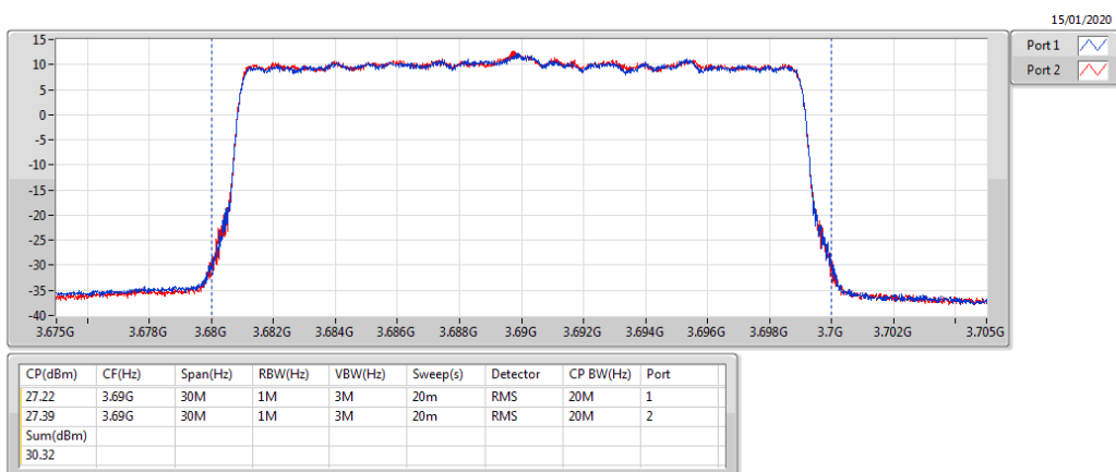
Band 48_LTE_20MHz_Nss1,16QAM_2TX 3690MHz_16QAM_RB 100,#RB 0
