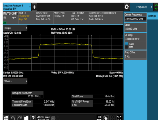
20M_Q16_FULLRB_OBW_Low channel
