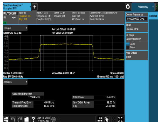
20M_QPSK_FULLLRB_OBW_High channel
