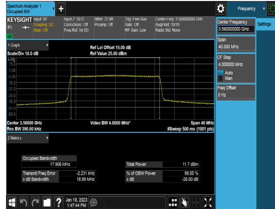
Ant 0_20M_QPSK_FULLLRB_OBW_High channel
