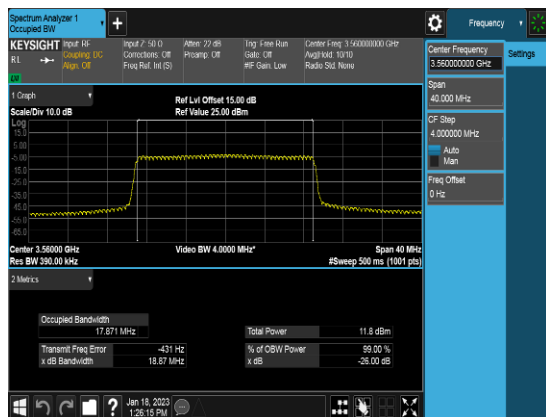
Ant 0_20M_QPSK_FULLLRB_OBW_Low channel
