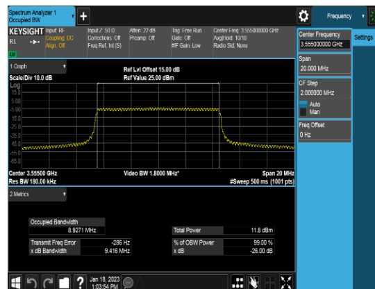
Ant 0_10M_Q64_FULLLRB_OBW_High channel
