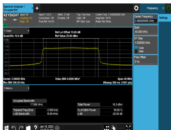
20M_QPSK_FULLLRB_OBW_Low channel
