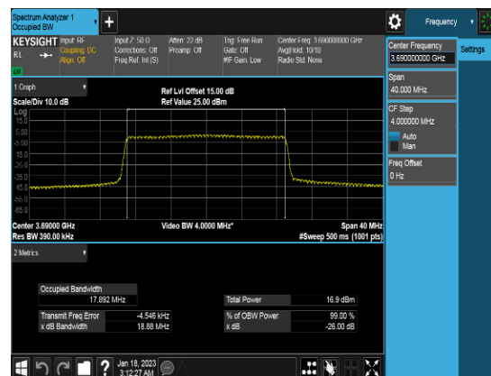
20M_Q16_FULLRB_OBW_Middle channel
