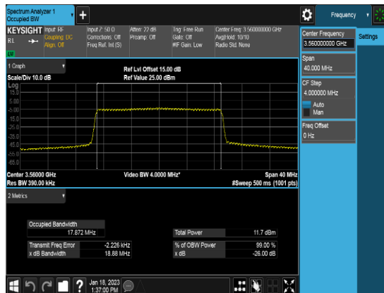
Ant 0_20M_Q16_FULLLRB_OBW_Low channel
