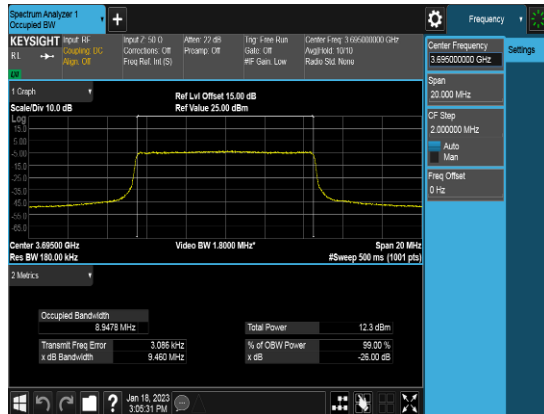
Ant 0_10M_QPSK_FULLLRB_OBW_Middle channel
