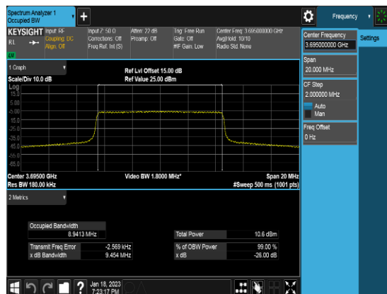
Ant 2_10M_Q16_FULLLRB_OBW_Middle channel
