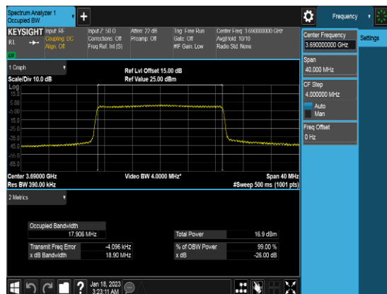
20M_Q64_FULLLRB_OBW_Middle channel
