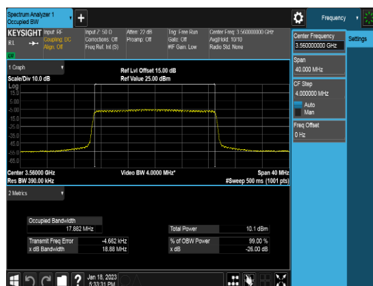
Ant 2_20M_QPSK_FULLLRB_OBW_Low channel
