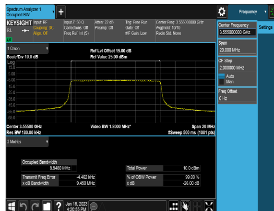
Ant 2_10M_Q64_FULLLRB_OBW_High channel
