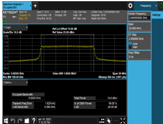
Ant 2_10M_QPSK_FULLLRB_OBW_Middle channel
