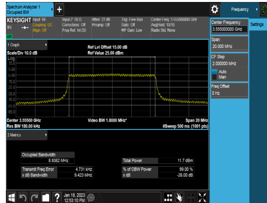
Ant 0_20M_Q16_FULLLRB_OBW_High channel
