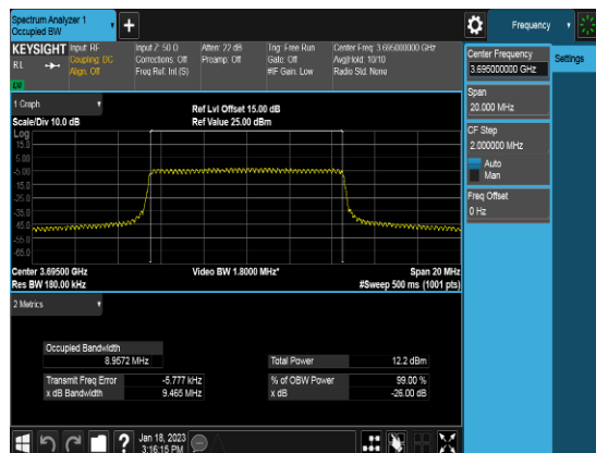
Ant 0_10M_Q16_FULLLRB_OBW_Middle channel
