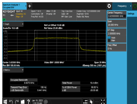
10M_Q64_FULLLRB_OBW_Low channel
