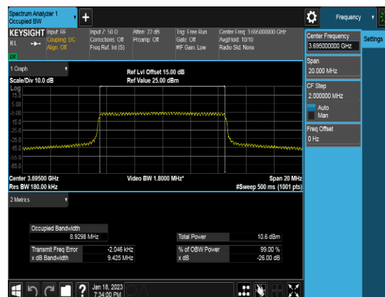
Ant 2_10M_Q64_FULLLRB_OBW_Middle channel
