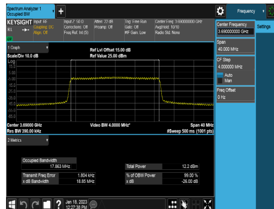
Ant 0_20M_Q16_FULLLRB_OBW_Middle channel
