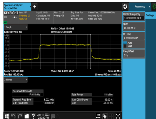
Ant 0_20M_QPSK_FULLLRB_OBW_Middle channel
