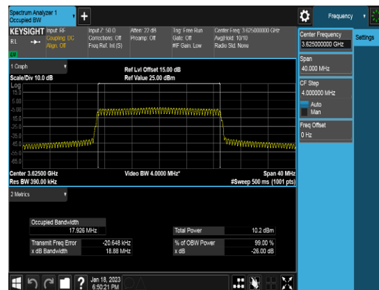
Ant 2_20M_Q16_FULLLRB_OBW_Middle channel
