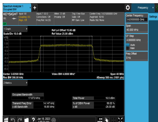
20M_QPSK_FULLLRB_OBW_Middle channel
