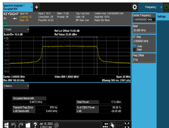
10M_Q16_FULLLRB_OBW_Middle channel
