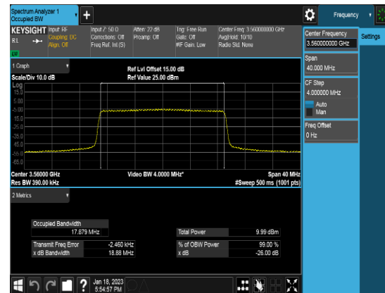
Ant 2_20M_QPSK_FULLLRB_OBW_High channel
