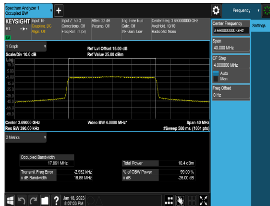
Ant 2_20M_Q64_FULLLRB_OBW_Middle channel
