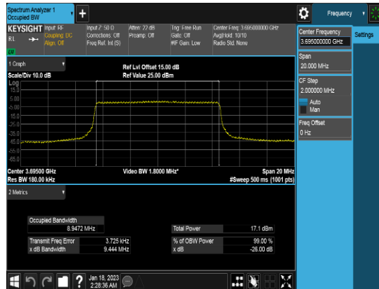
10M_QPSK_FULLRB_OBW_Middle channel
