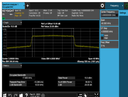
SCC_20M_3690MHz_Q64_FULLLRB_OBW
