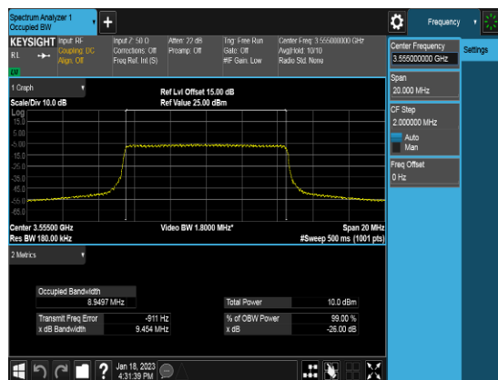
Ant 2_10M_Q64_FULLLRB_OBW_Low channel
