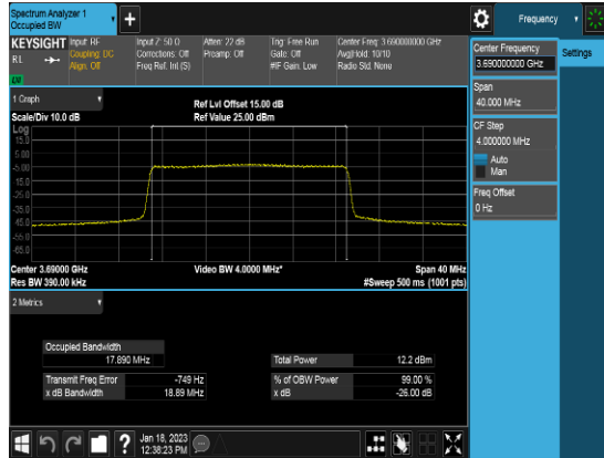
Ant 0_20M_Q64_FULLLRB_OBW_Middle channel
