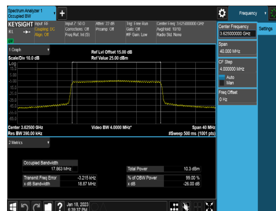
Ant 2_20M_QPSK_FULLLRB_OBW_Middle channel
