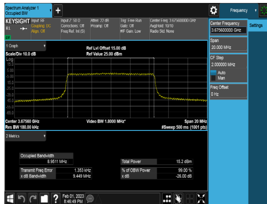
PCC_10M_3675.6MHz_QPSK_FULLLRB_OBW
