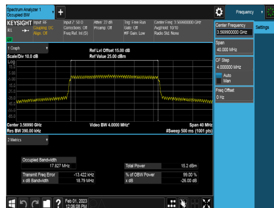
SCC_20M_3569.9MHz_QPSK_FULLLRB_OBW
