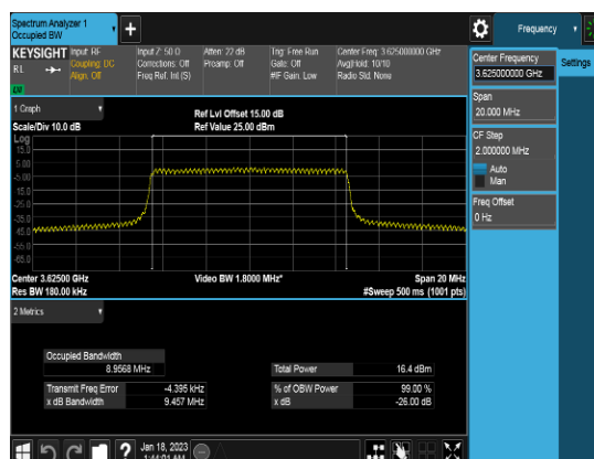
10M_Q64_FULLLRB_OBW_Middle channel
