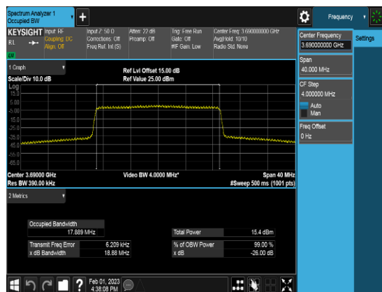
SCC_20M_3690MHz_Q64_FULLLRB_OBW
