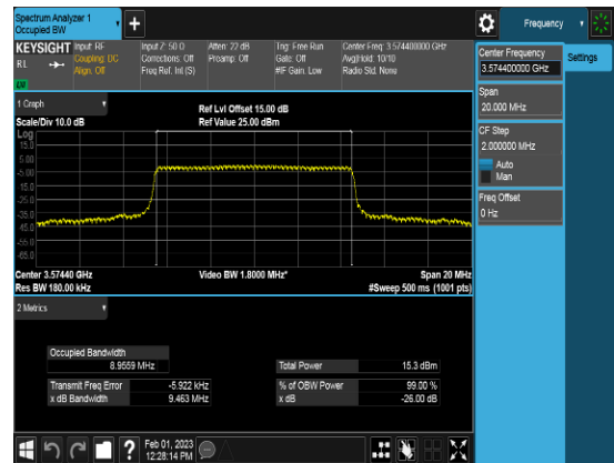
SCC_10M_3574.4MHz_QPSK_FULLLRB_OBW
