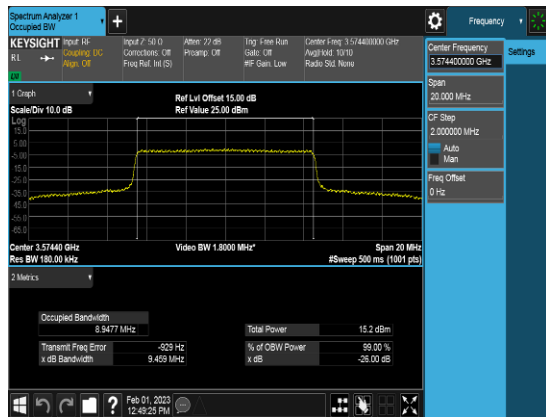
SCC_10M_3574.4MHz_Q64_FULLLRB_OBW
