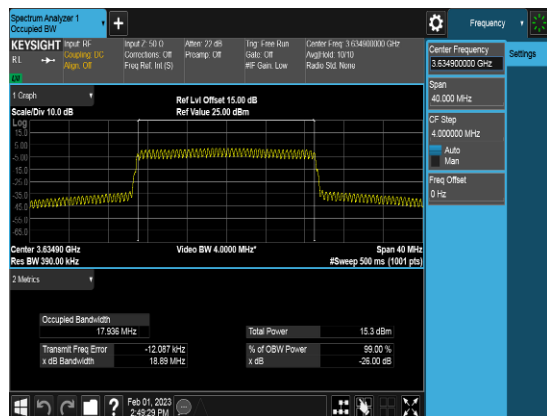
SCC_20M_3634.9MHz_QPSK_FULLLRB_OBW
