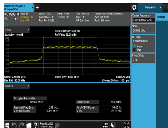
SCC_10M_3694.5MHz_QPSK_FULLLRB_OBW
