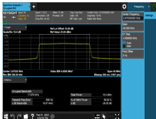
PCC_20M_3670.2MHz_QPSK_FULLLRB_OBW
