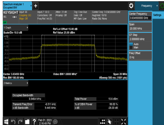
SCC_10M_3634.5MHz_QPSK_FULLLRB_OBW
