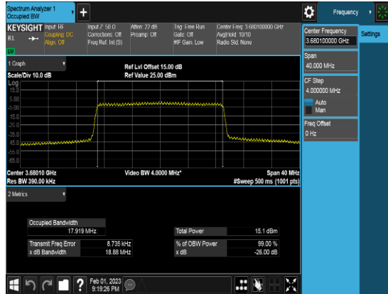
PCC_20M_3680.1MHz_QPSK_FULLLRB_OBW
