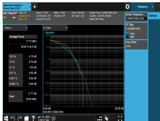
20M_Q64_1RB0_PAPR_Middle channel
