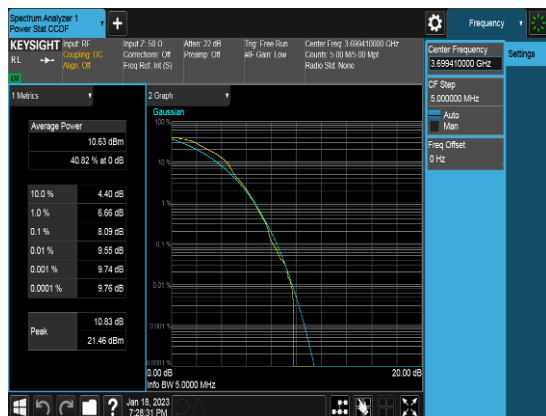
Ant 2_10M_Q16_1RB0_PAPR_Middle channel
