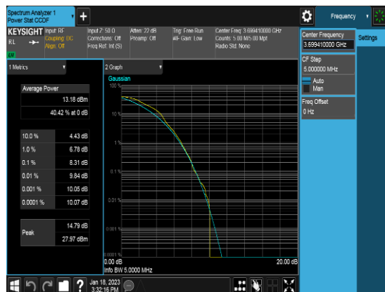
Ant 0_10M_Q64_1RB0_PAPR_Middle channel
