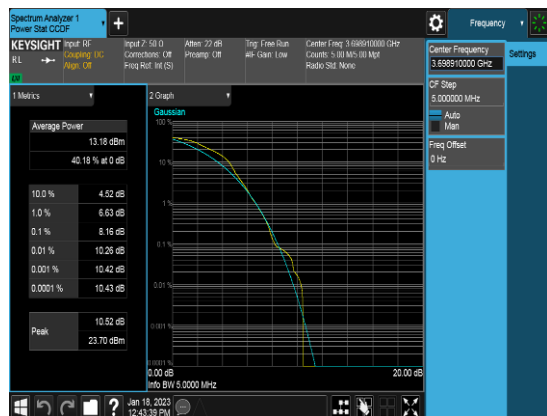
Ant 0_20M_Q64_1RB0_PAPR_Middle channel
