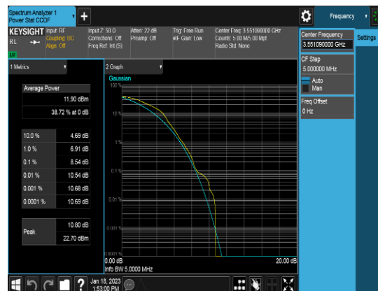
Ant 0_20M_Q64_FULLRB_PAPR_High channel
