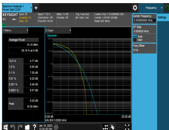
Ant 0_10M_QPSK_FULLRB_PAPR_Low channel
