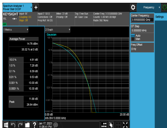
10M_Q64_FULLRB_PAPR_Low channel
