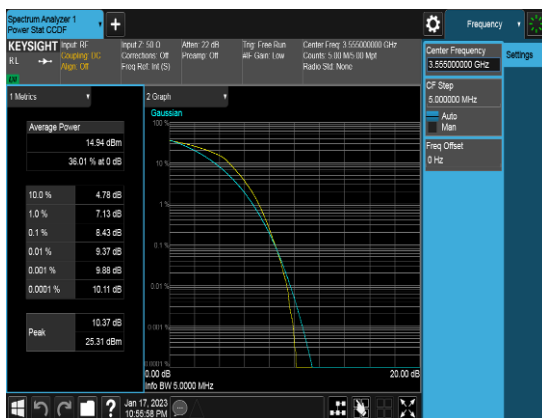
10M_Q16_FULLRB_PAPR_Low channel
