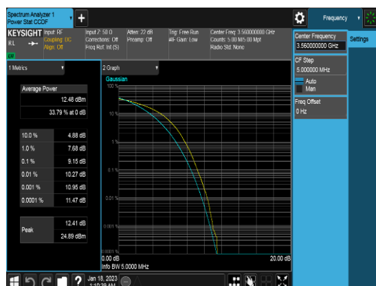
20M_Q64_FULLRB_PAPR_Low channel
