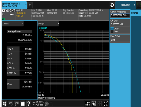
20M_Q16_1RB0_PAPR_Middle channel
