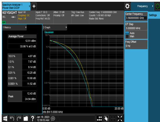
20M_Q16_FULLRB_PAPR_Low channel
