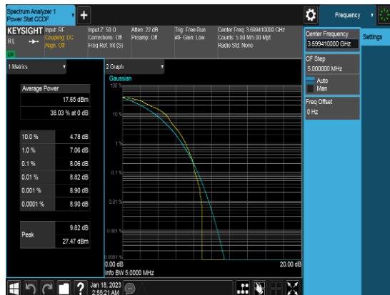
10M_Q64_1RB0_PAPR_Middle channel
