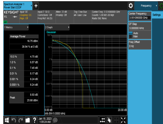
20M_Q16_FULLRB_PAPR_High channel
