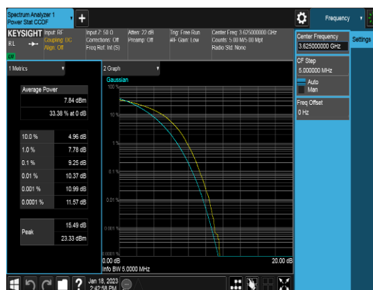
Ant 0_20M_Q16_FULLRB_PAPR_Middle channel
