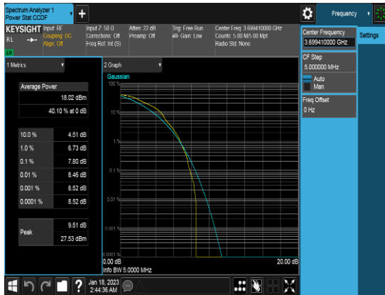
10M_Q16_1RB0_PAPR_Middle channel
