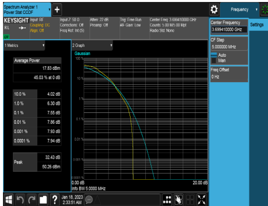
10M_QPSK_1RB0_PAPR_Middle channel
