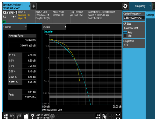
10M_Q64_FULLRB_PAPR_High channel
