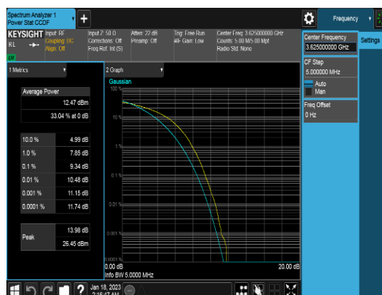
20M_Q64_FULLRB_PAPR_Middle channel
