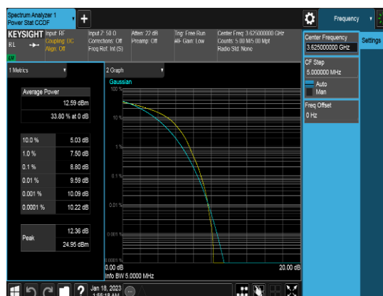
20M_QPSK_FULLRB_PAPR_Middle channel
