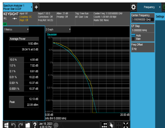
Ant 2_10M_Q16_FULLRB_PAPR_High channel
