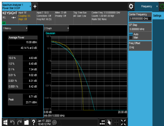
10M_QPSK_FULLRB_PAPR_Low channel
